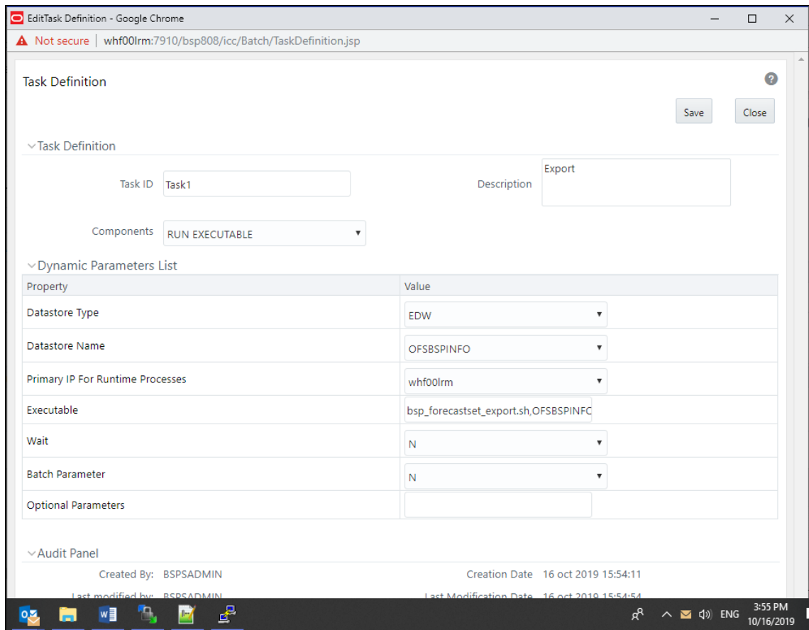
Figure 24: Batch Maintenance
