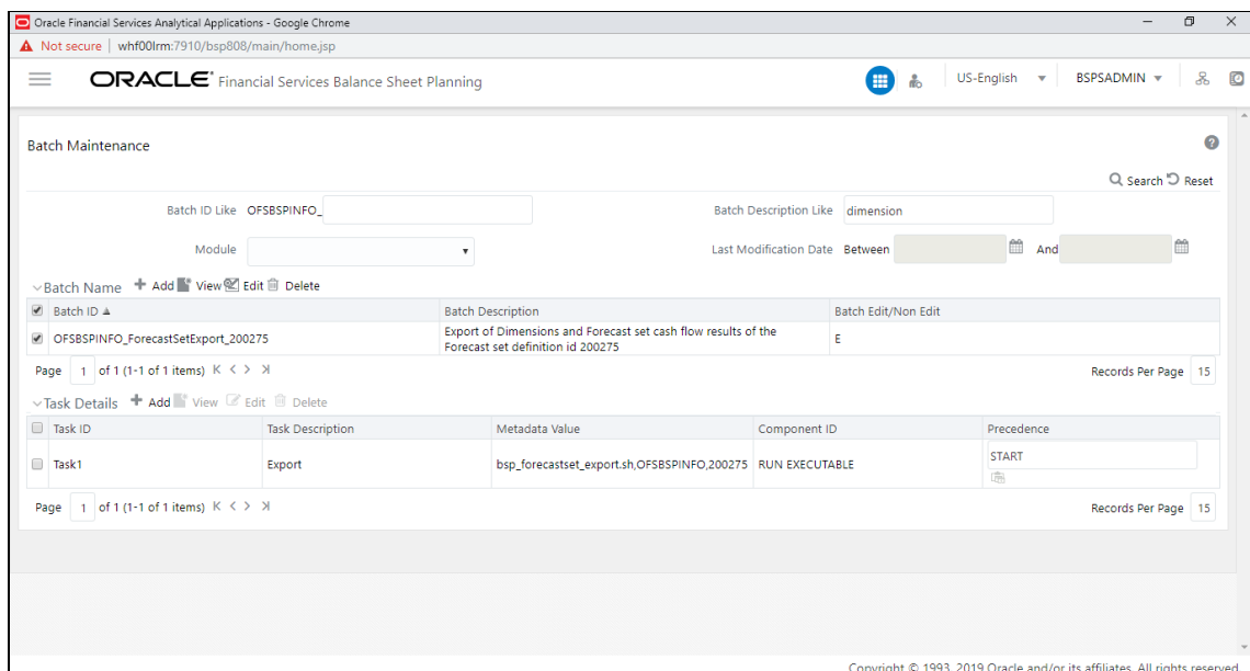
Figure 24: Batch Maintenance
