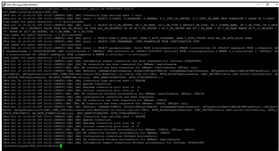
Figure 19: Putty screen 2
