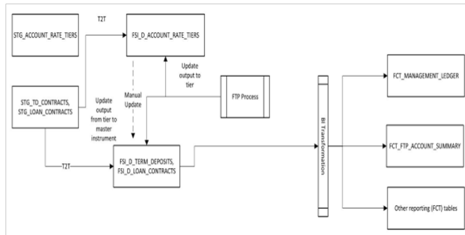
FTP Data Flow
