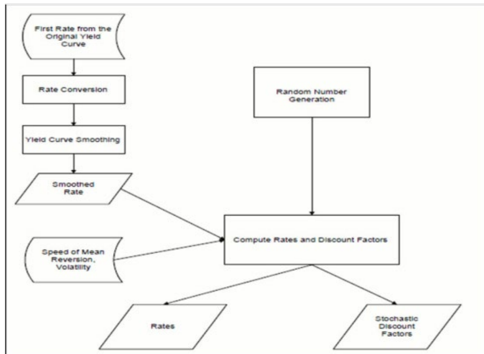
Process flow for Vasicek (or Merton) models
