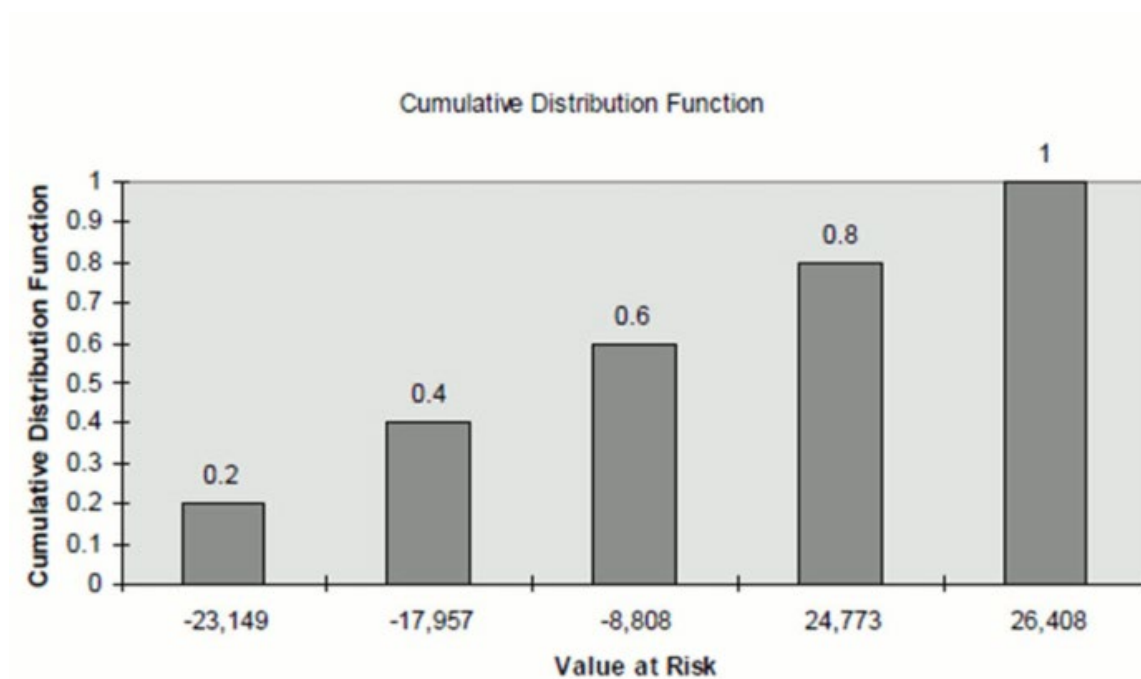
Graph of cumulative distribution function
