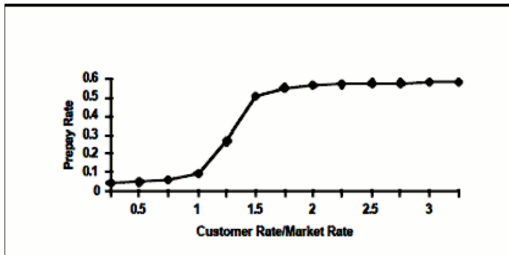
Figure 1: Graph between Market Rate and Prepayment Rule
