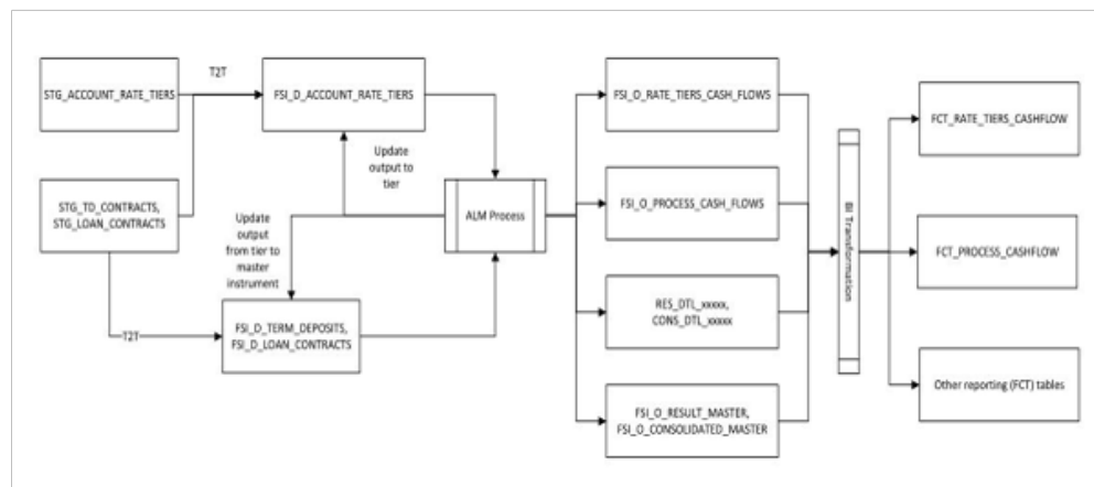
ALM Data Flow
