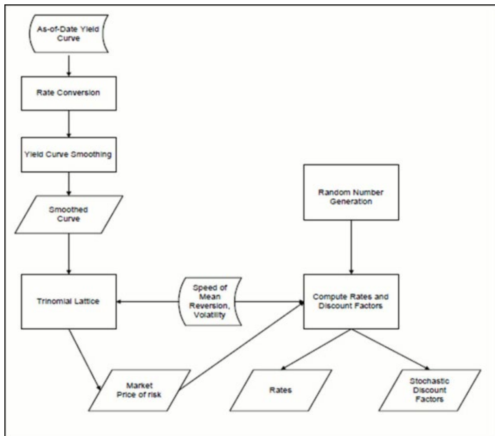
Process flow for Extended Vasicek and Ho & Lee
