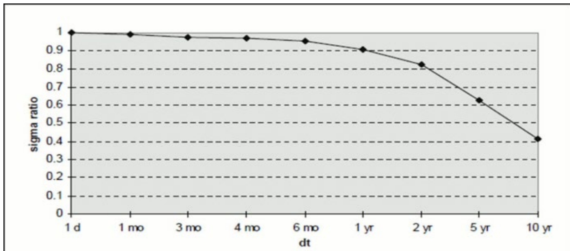
Graph of change in the ratio \sigma_{1m} / \sigma_i varying \Delta t ( \alpha_i = 0.1 )
