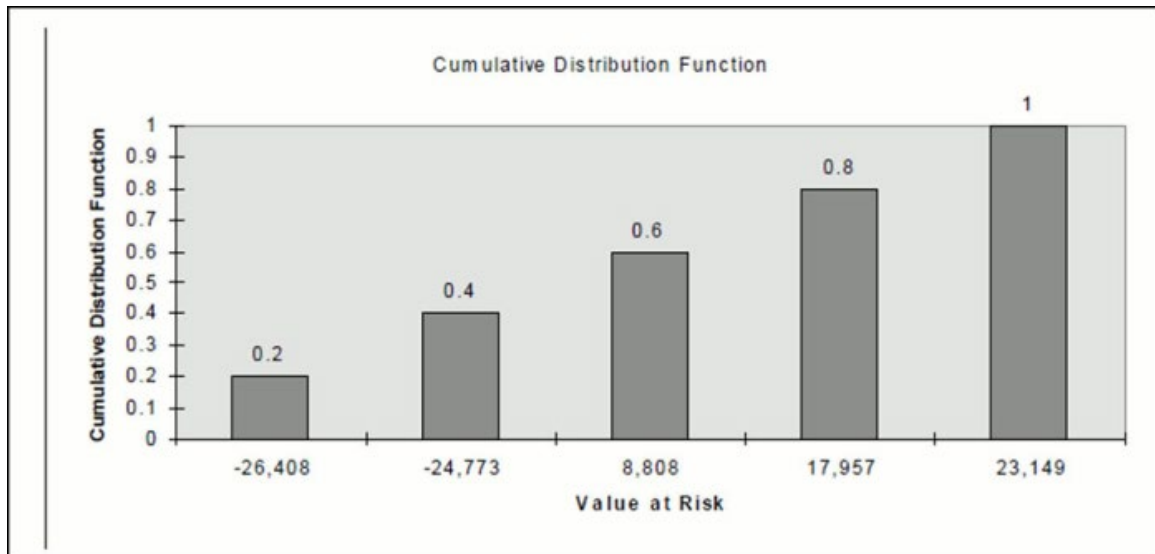
Graph of cumulative distribution function
