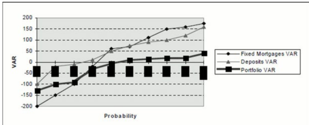
Graph for Output From Monte Carlo
