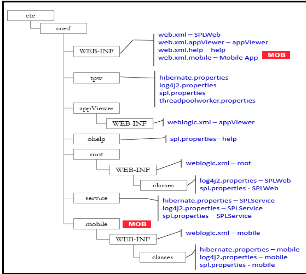
Figure 21: Configuration File Hierarchy
