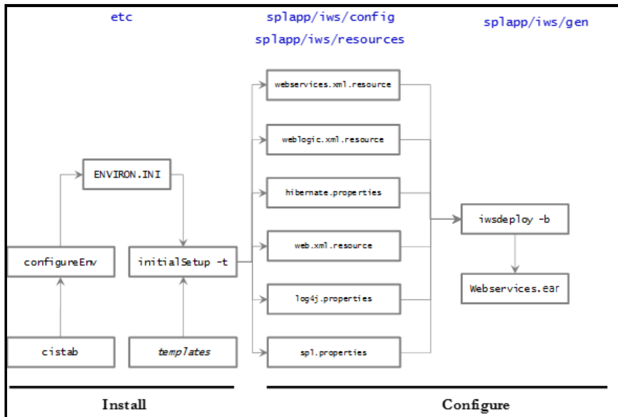
Figure 26: Inbound Web Services Configuration Process
