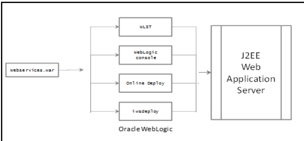
Figure 27: Inbound Web Services Deployment Process
