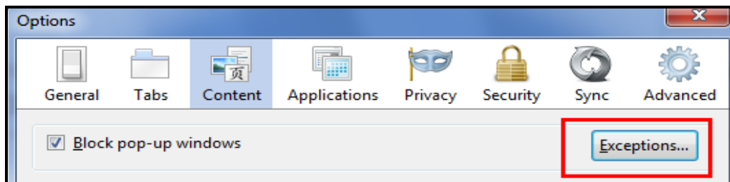
Figure 23: Exceptions
