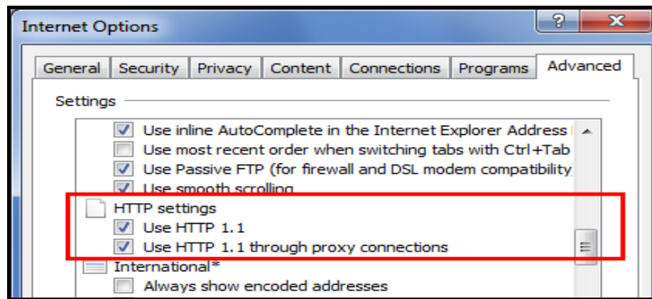
Figure 20: HTTP 1.1 Settings
