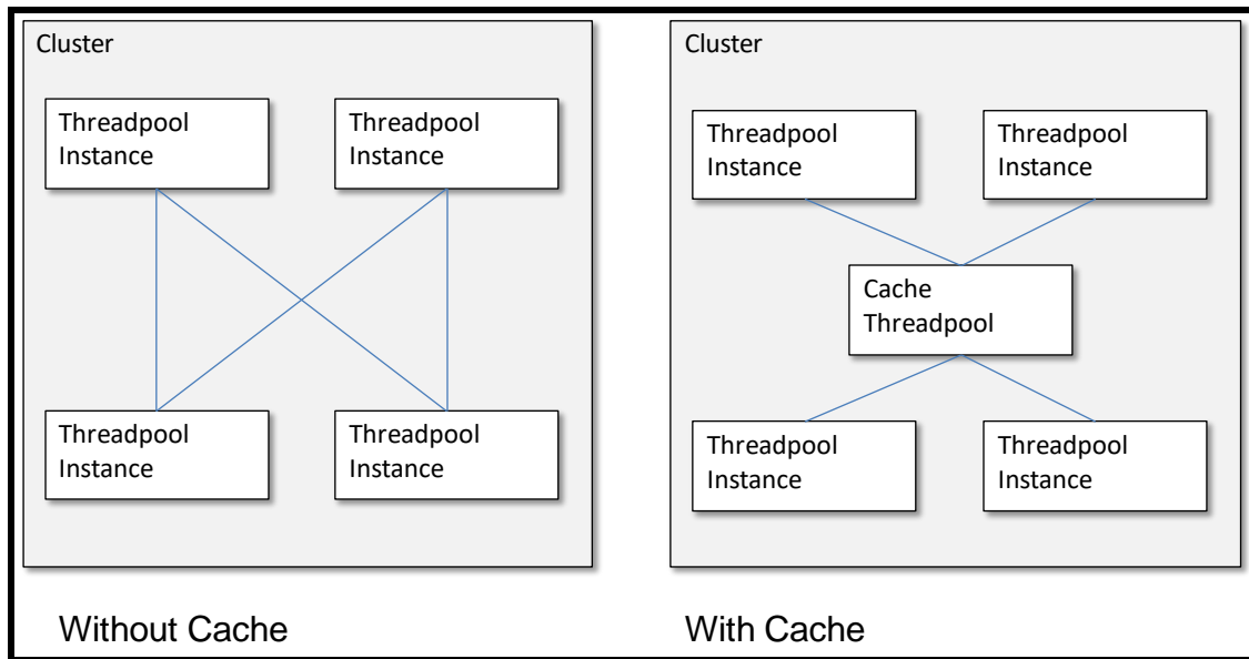
Figure 40: Cache Architecture
