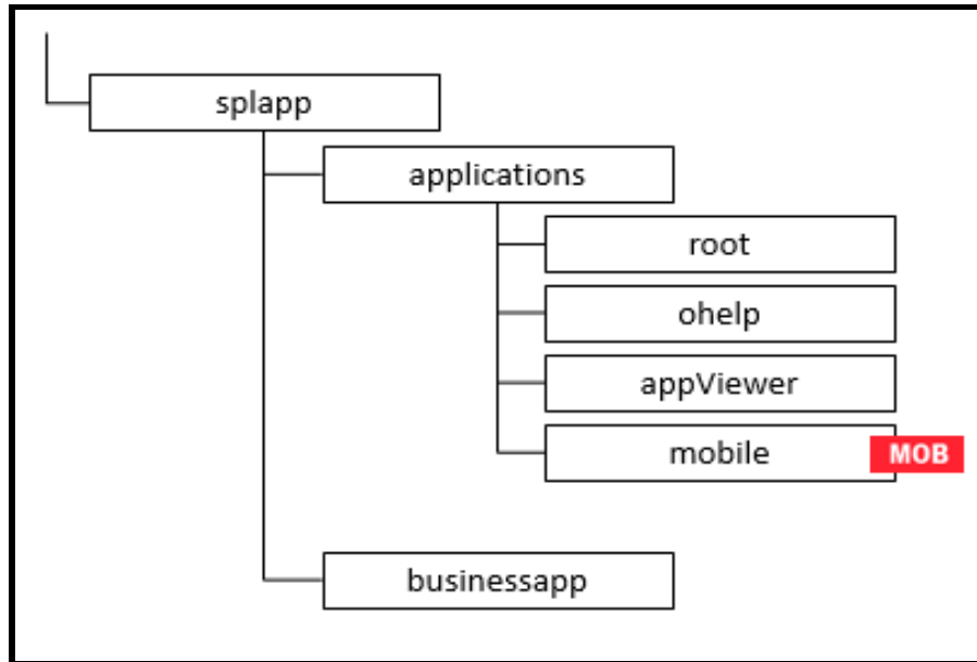
Figure 42: Expanded Format
