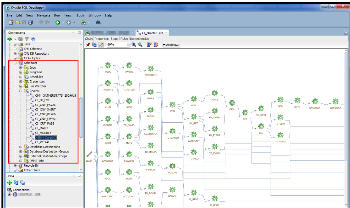
Figure 38: Example Oracle SQL Developer Oracle Scheduler Interface
