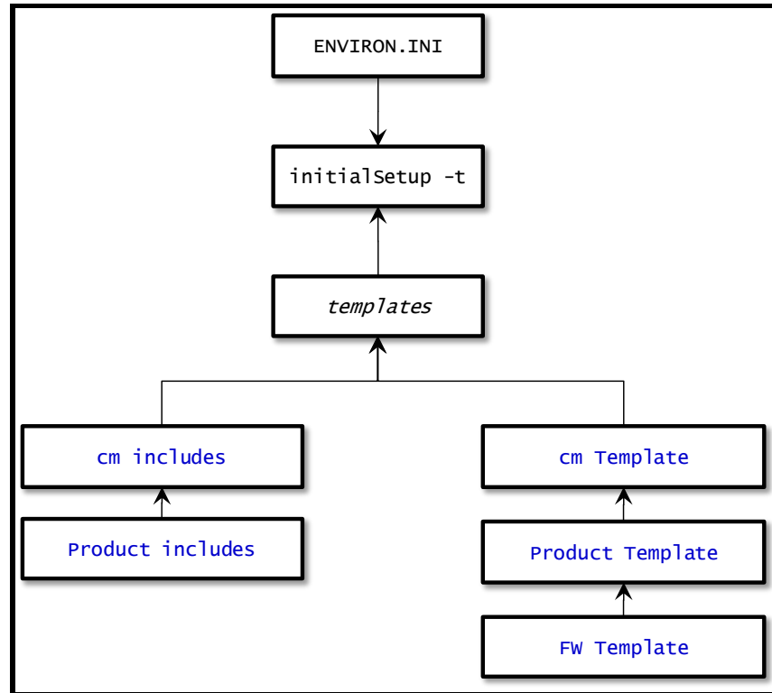
Figure 33: Template Hierarchy
