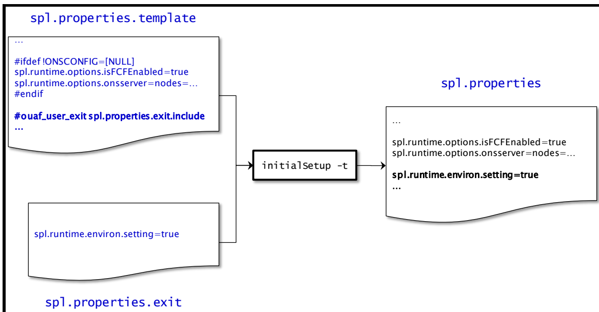
Figure 32: Include Files
