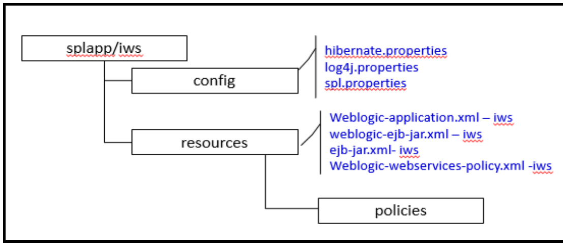
Figure 32: Inbound Web Services Configuration
