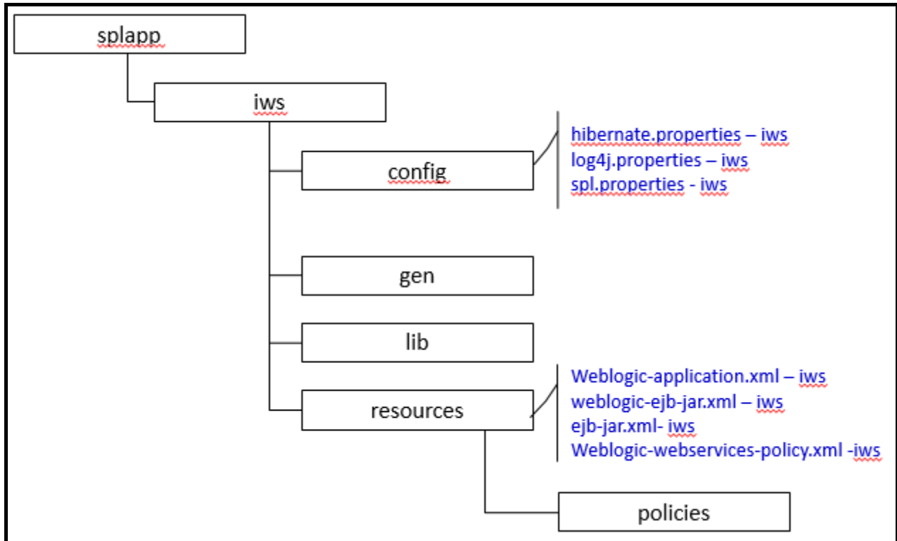
Figure 33: Inbound Web Services Structures
