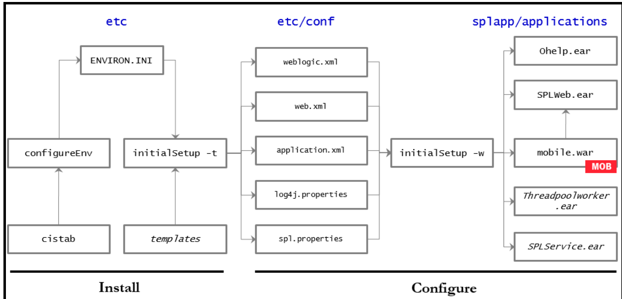
Figure 22: Web Application Server Configuration Process
