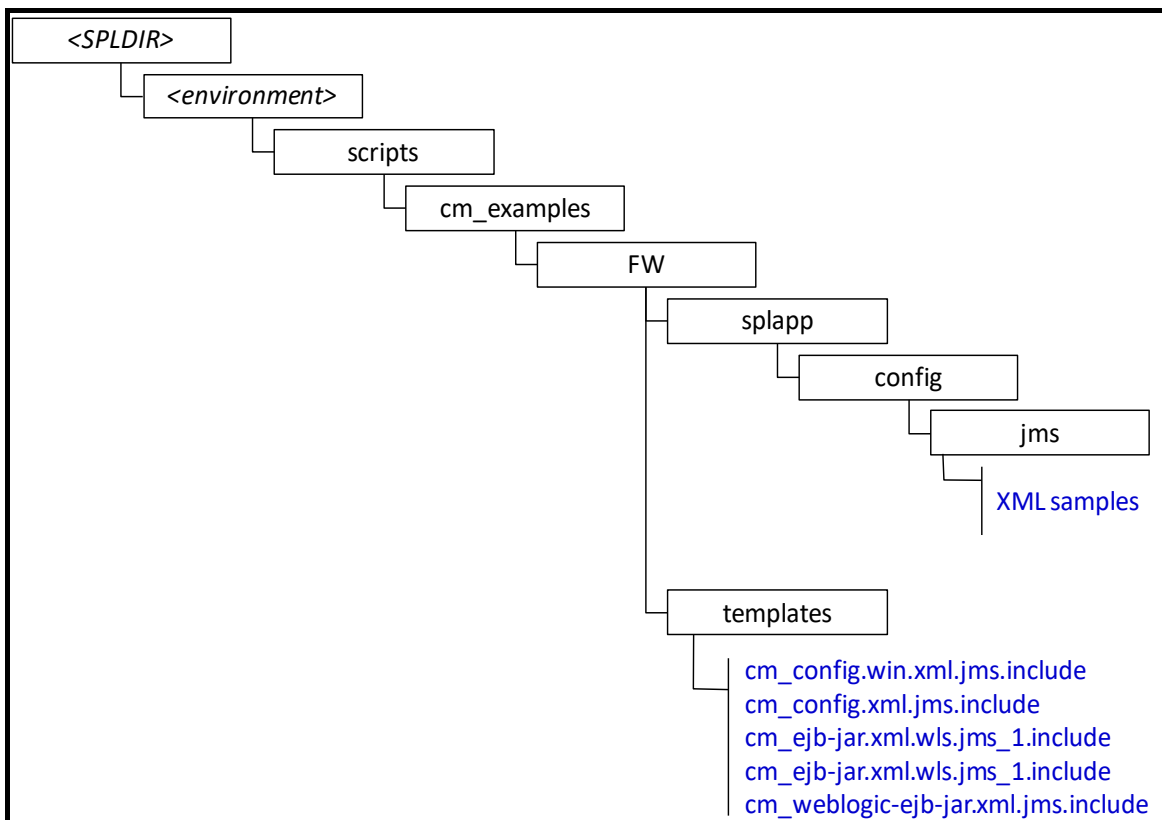
Figure 34: Custom JMS Configuration
