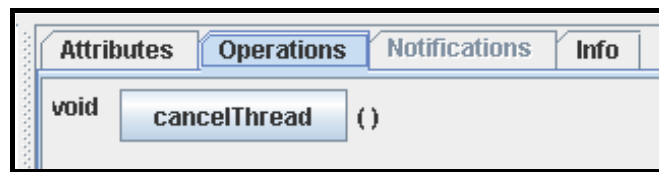
Figure 50: CancelThread Example
