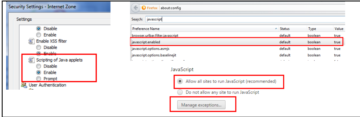
Figure 191: Javascript Settings
