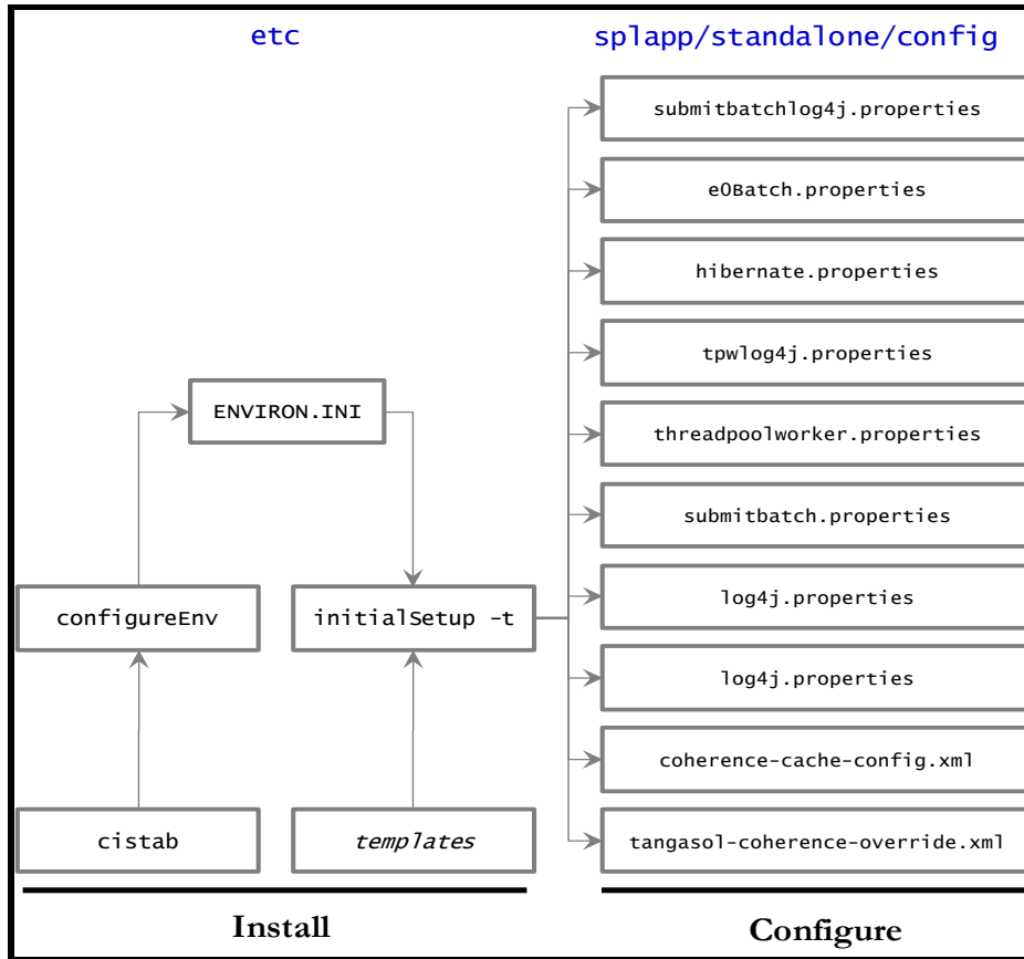
Figure 30: Batch Configuration Process
