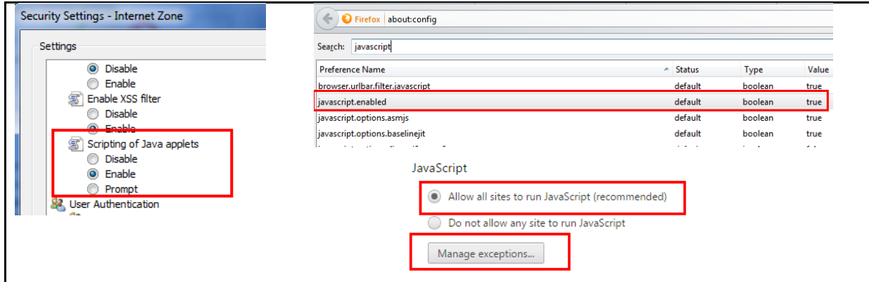
Figure 22: Javascript Settings
