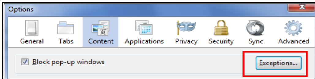
Figure 24: Exceptions
