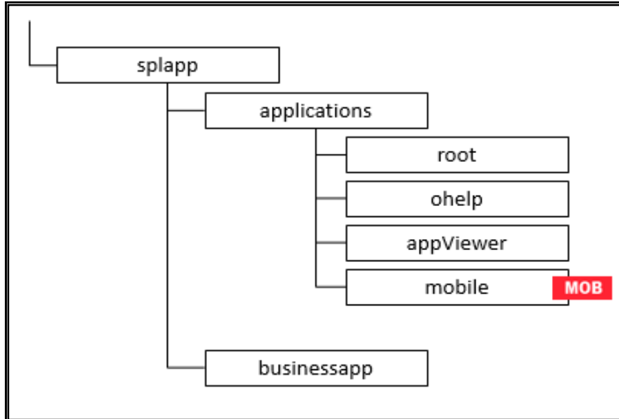
Figure 43: Expanded Format
