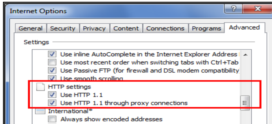
Figure 21: HTTP 1.1 Settings
