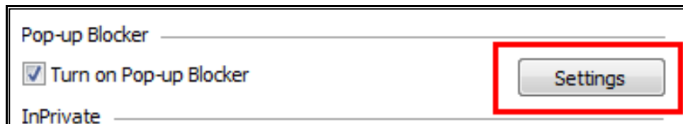
Figure 23: Pop-up Blocker
