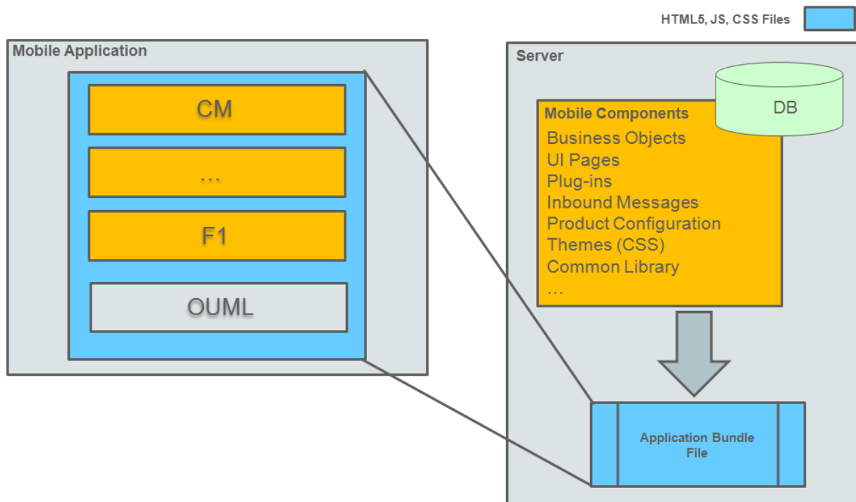
Figure 6: Mobile Application Bundle
