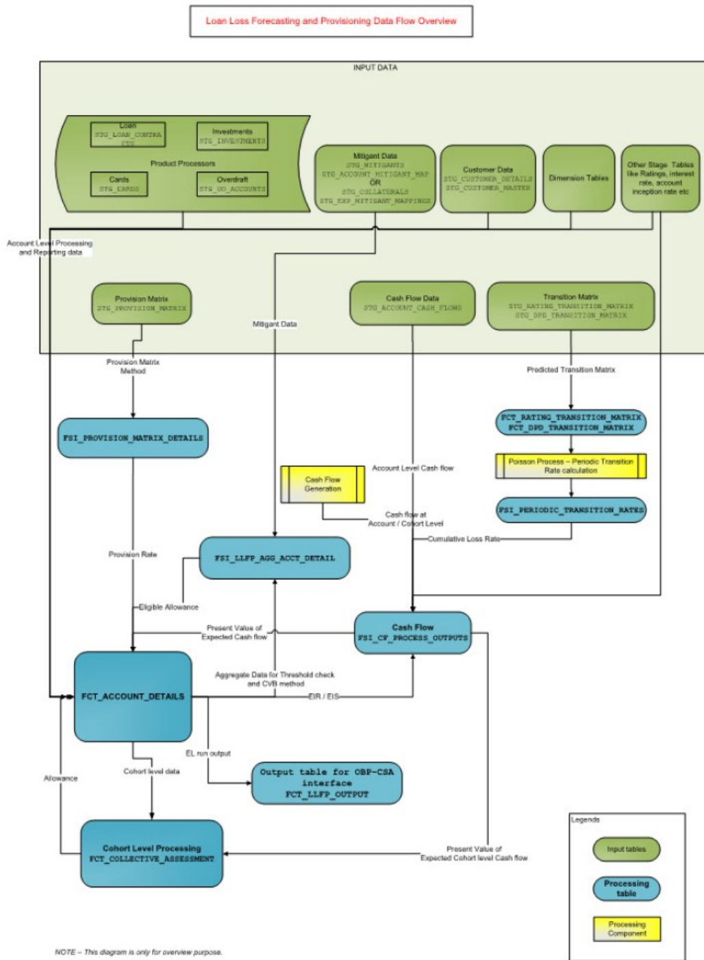
Figure 135: The LLFP Application Data Flow
