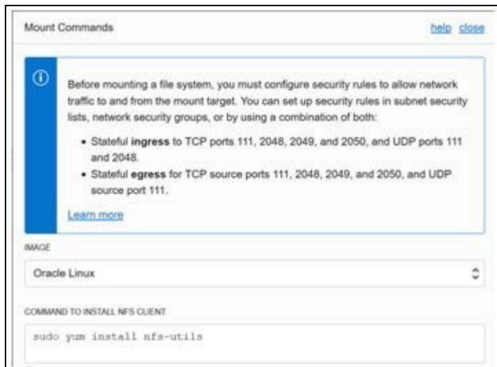
Figure 19: The Mount Commands Window
