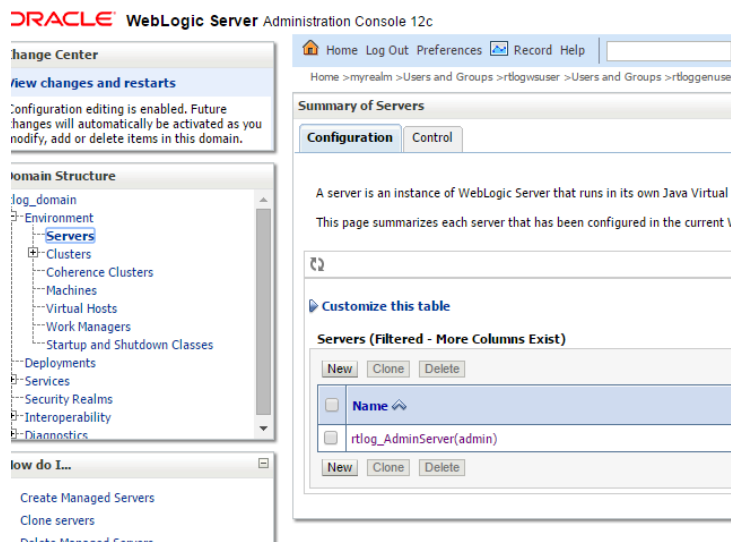
Figure 6–39 Administration Console Servers Page
