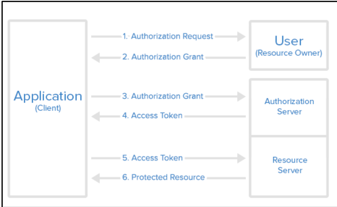
Figure 1: JWT Roles
