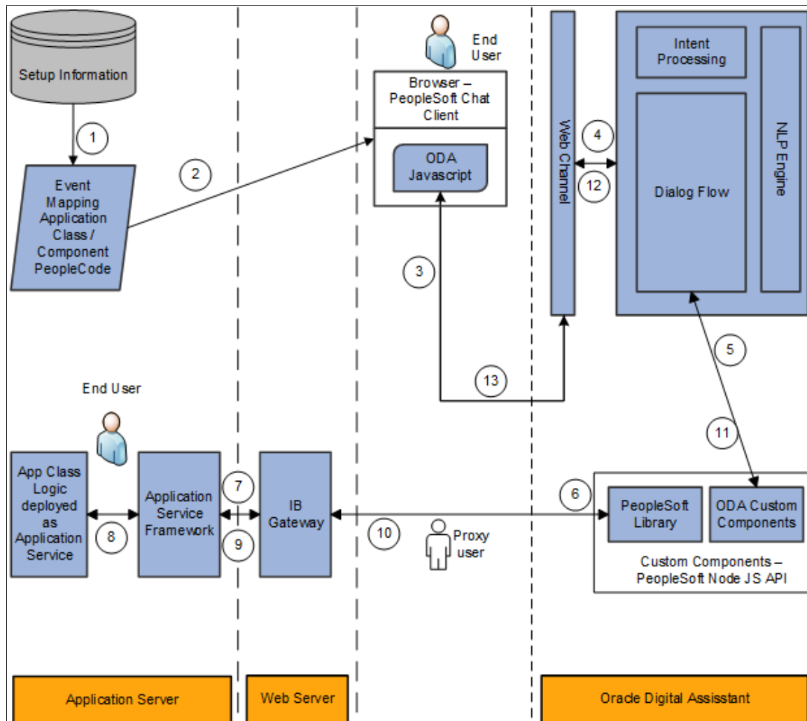
Chatbot Architecture Diagram
