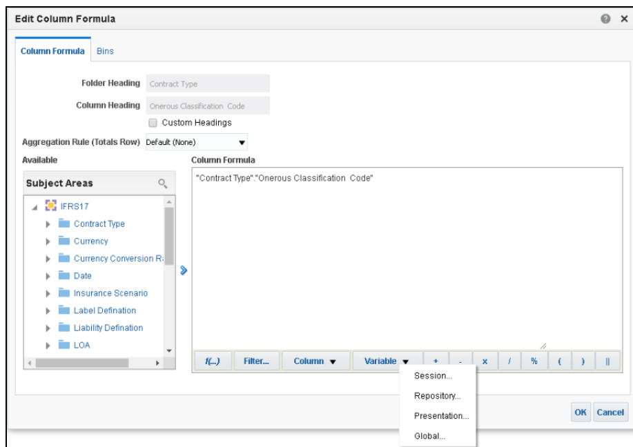
Figure 27: The Edit Column Formula
