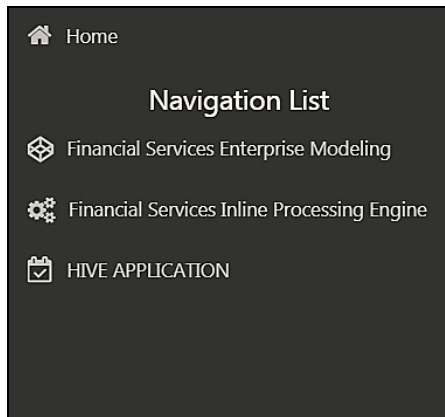
Figure 18: Navigation Drawer
