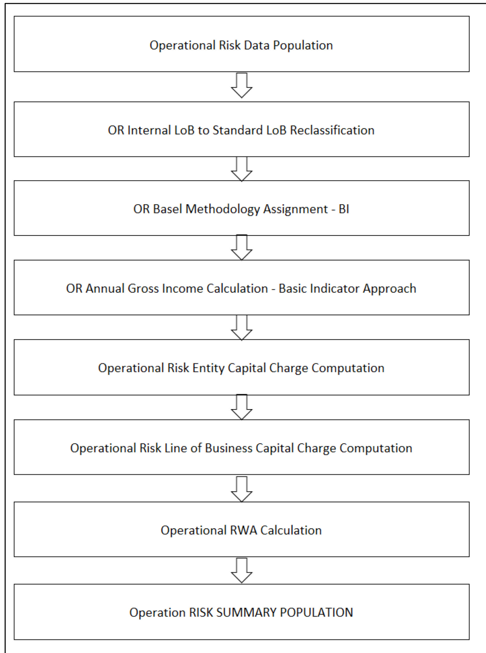
Figure 43: Operational Risk-Basic Indicator Approach - Data Population
