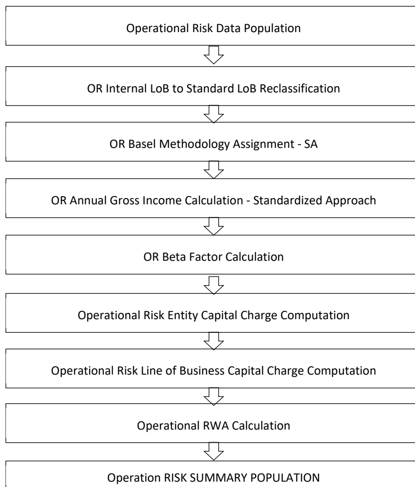
Figure 44: Process Flow for Operational Risk-Standardized Approach - Data Population
