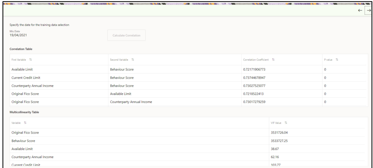
Figure 103: Training Data Selection for Account Clustering Model Definition
