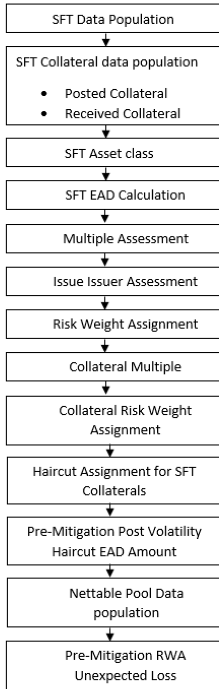
Figure 36: Process Flow for Credit Risk Securities Financing Transactions
