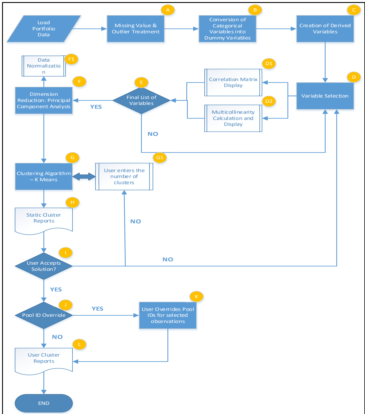
Figure 100: Process Flow for Account Clustering
