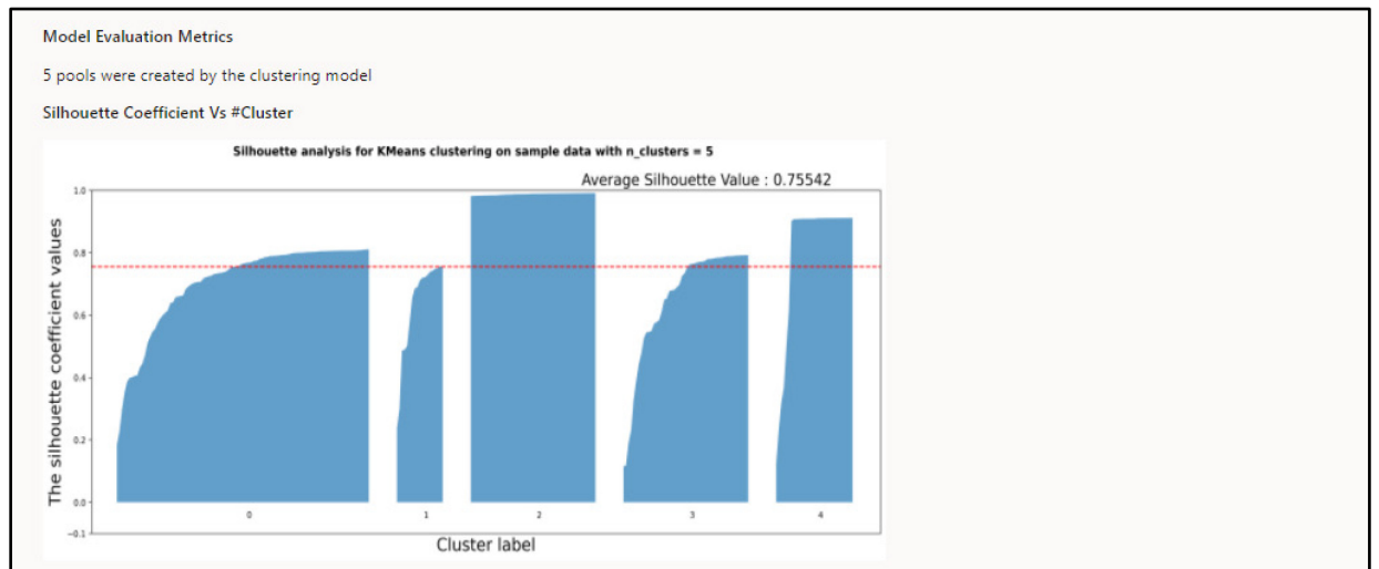
Figure 104: Model Evaluation Metrics
