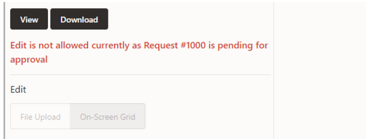
Figure 119: Error message
