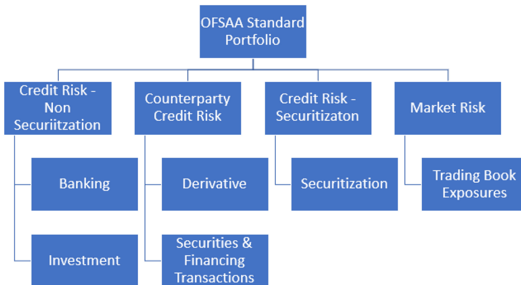
Figure 21: High-level design
