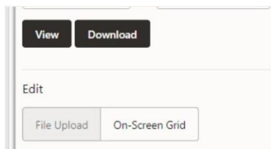
Figure 116: On-Screen grid
