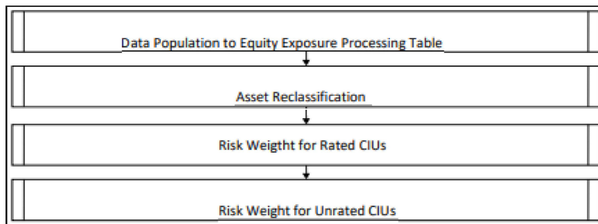
Figure 33: Processing CIU
