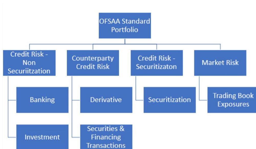
Figure 21: High-level design
