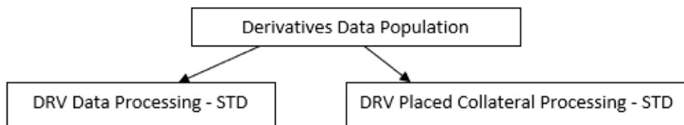
Figure 24: Derivative portfolio
