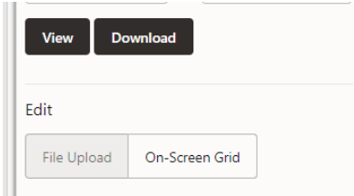
Figure 34: On-Screen grid
