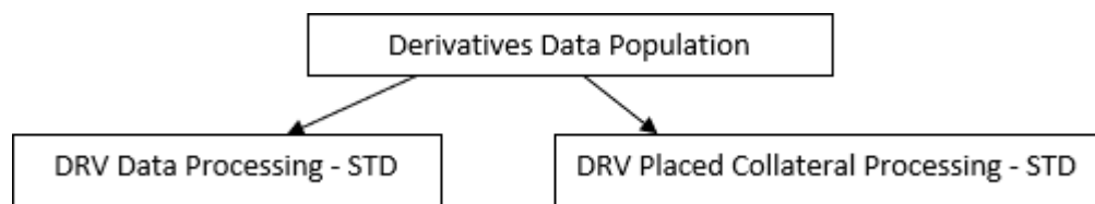
Figure 5: Derivative portfolio
