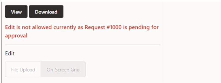
Figure 37: Error message
