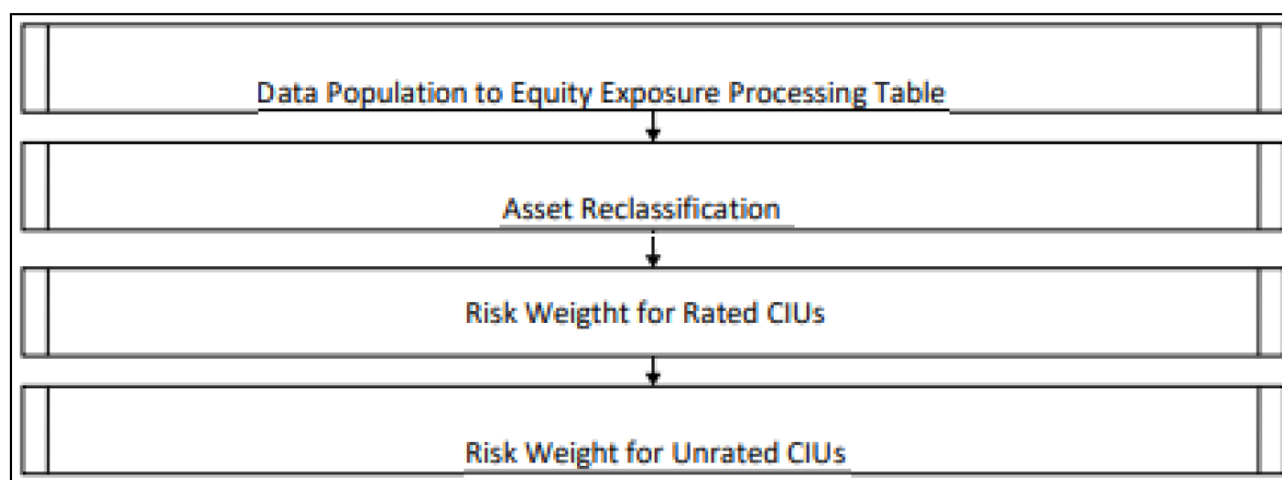
Figure 14: Processing CIU
