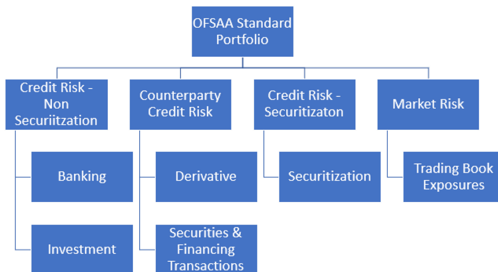
Figure 20: OFSAA profile
