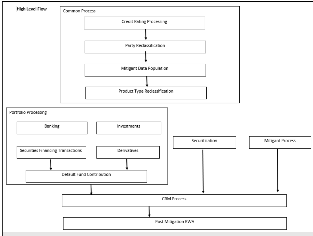
Figure 21: High-level design
