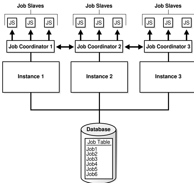
Figure 27-7 Oracle RAC Architecture and the Scheduler
