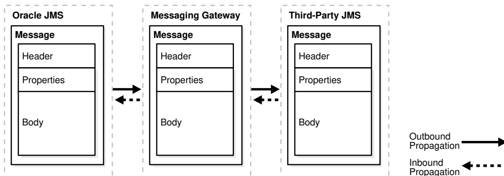
Figure C-6 JMS Message Propagation
