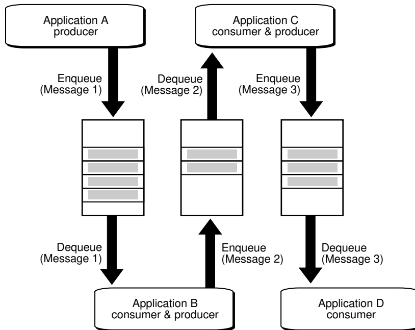
Figure 1-5 Implementing a Workflow using TEQ and AQ
