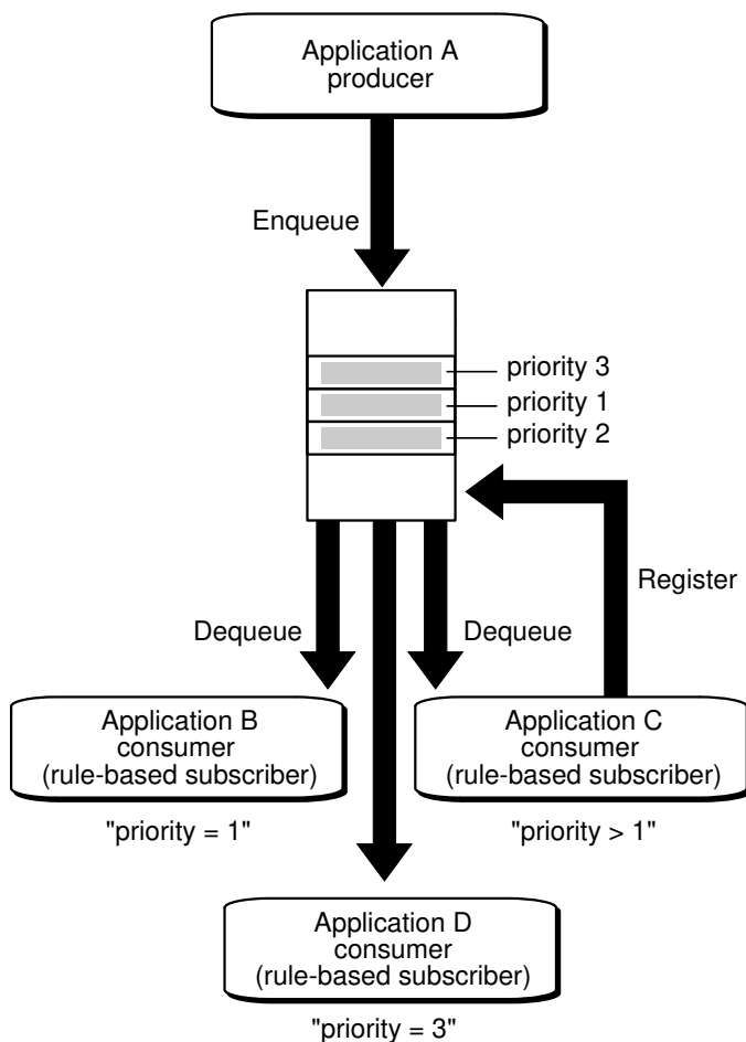
Figure 1-8 Implementing Publish/Subscribe using TEQ and AQ
