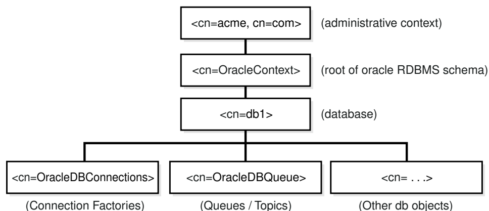
Figure 7-1 Structure of Oracle Database Advanced Queuing Entries in LDAP Server
