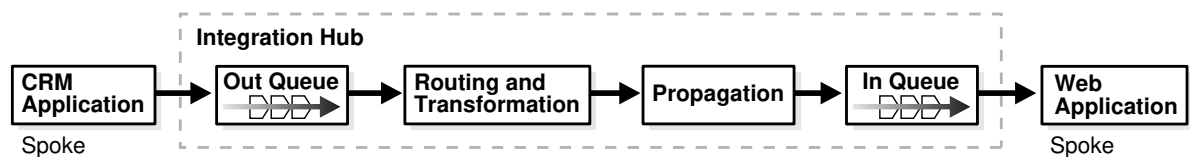
Figure 1-10 Transformations in Application Integration
