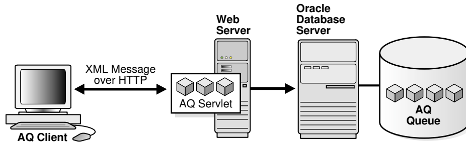
Figure 1-11 Architecture for Performing Oracle Database Advanced Queuing Operations Using HTTP
