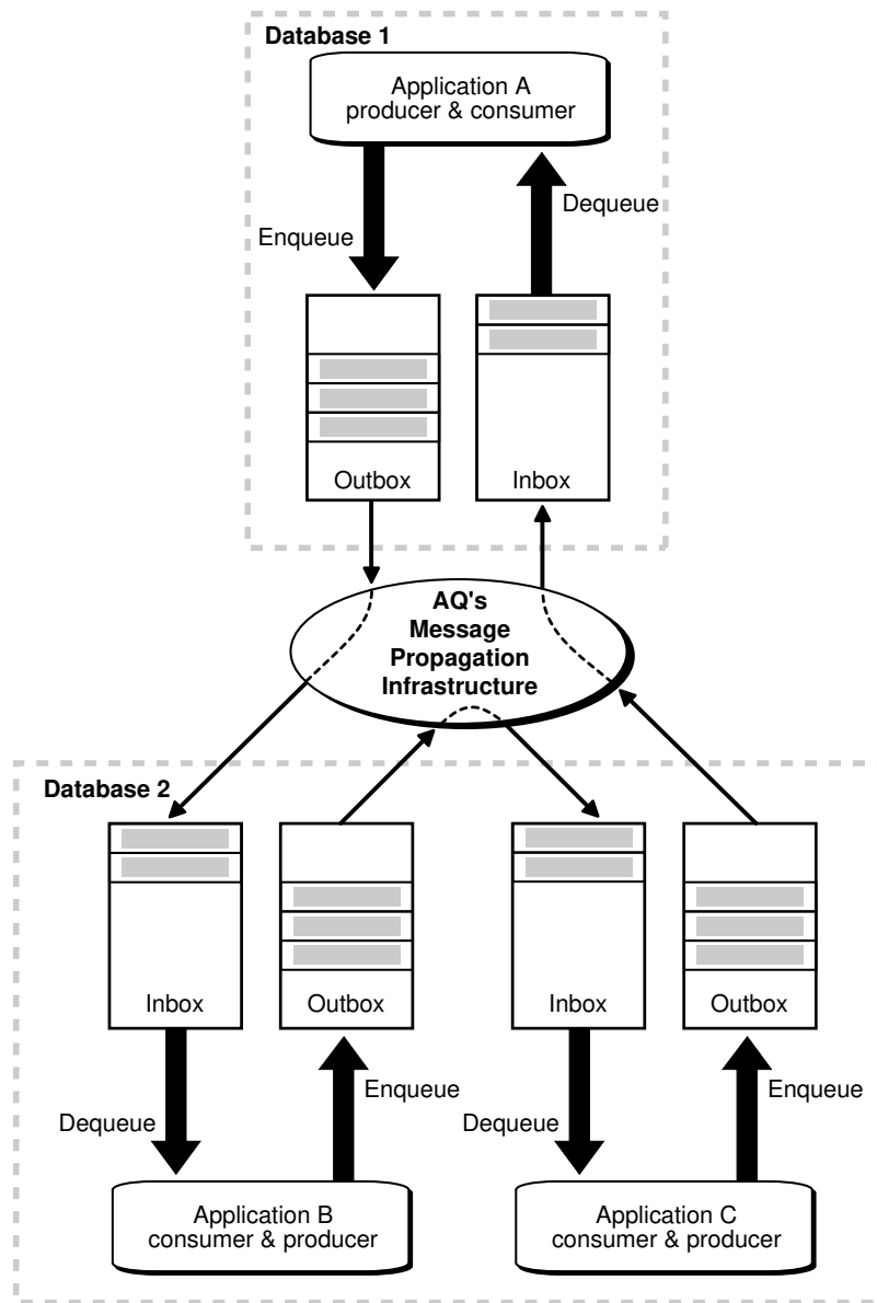
Figure 1-9 Message Propagation in Oracle Database Advanced Queuing
