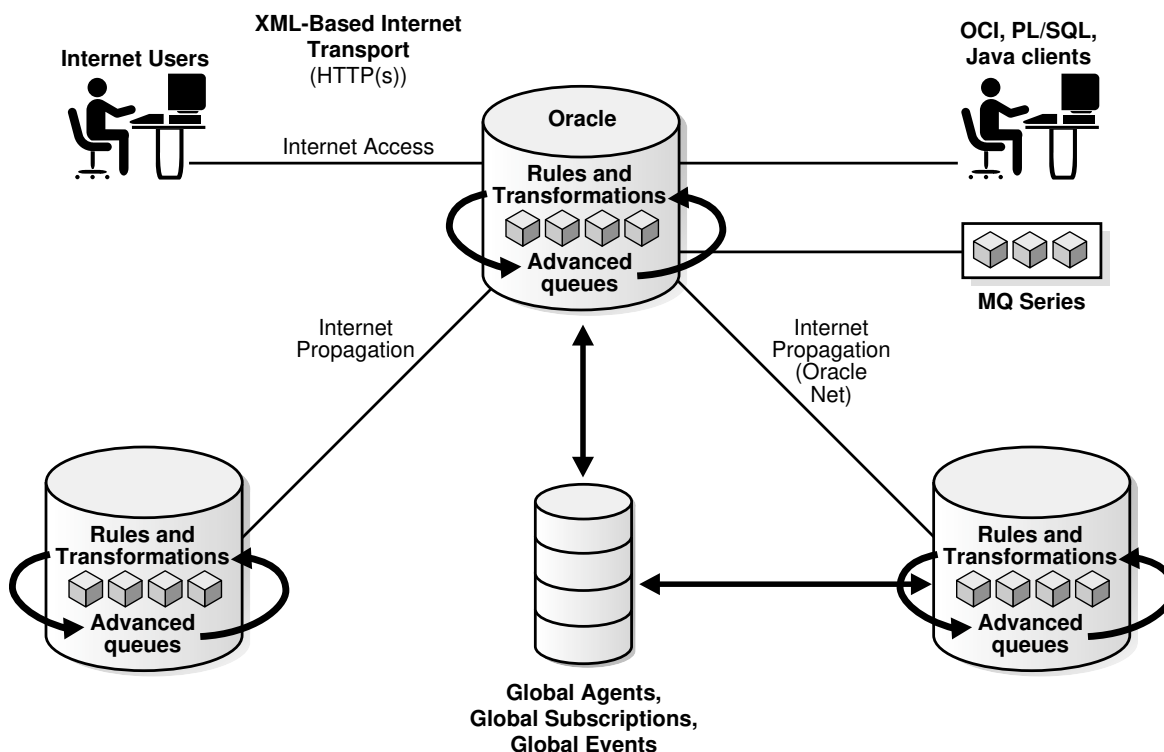
Figure 1-1 Integrated Application Environment Using TEQ and AQ
