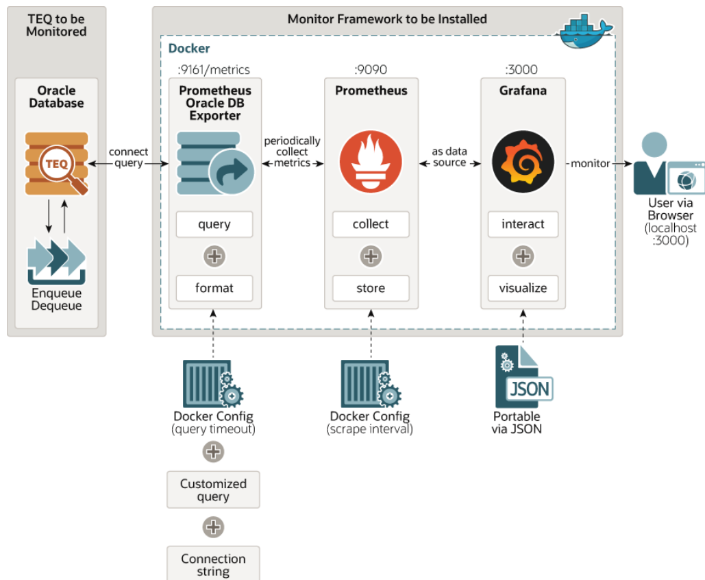
Figure 11-1 Monitoring Transaction Event Queue
