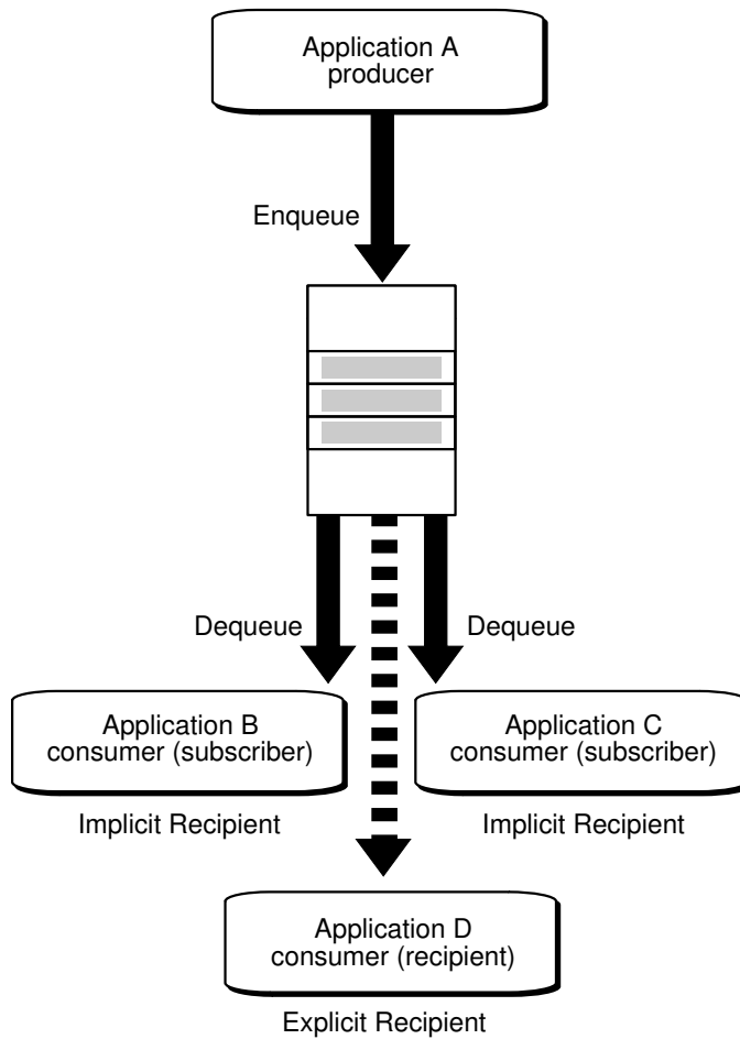
Figure 1-4 Explicit and Implicit Recipients of Messages
