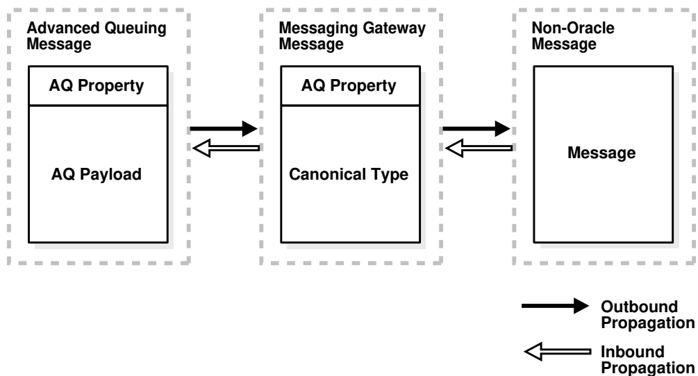
Figure C-2 Non-JMS Message Conversion
