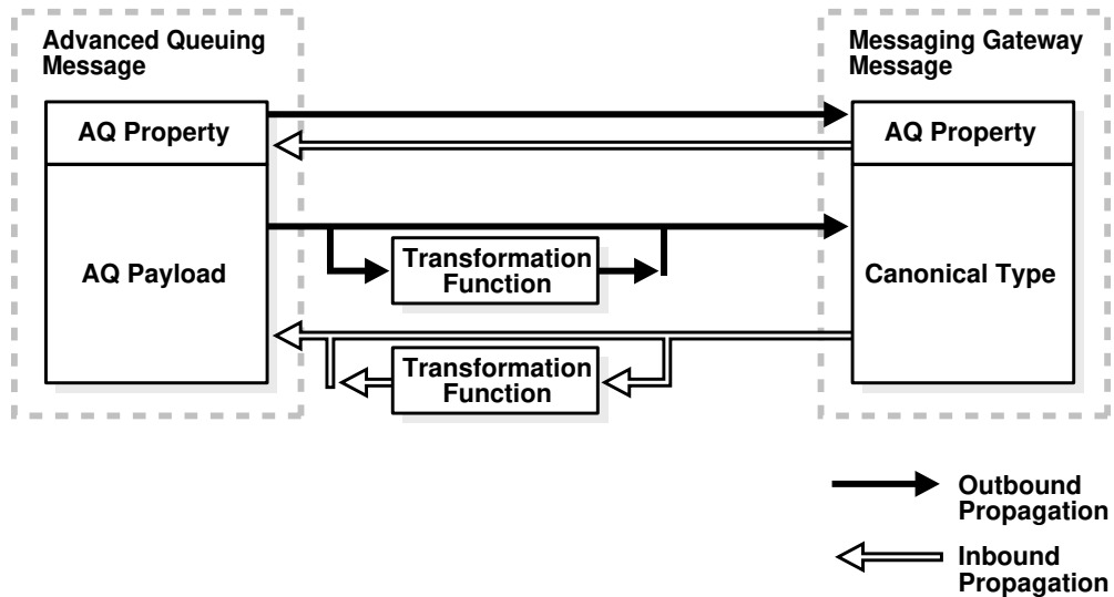
Figure C-3 Oracle Database Advanced Queuing Message Conversion
