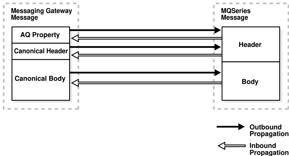
Figure C-4 Message Conversion for WebSphere MQ Using MGW_BASIC_MSG_T
