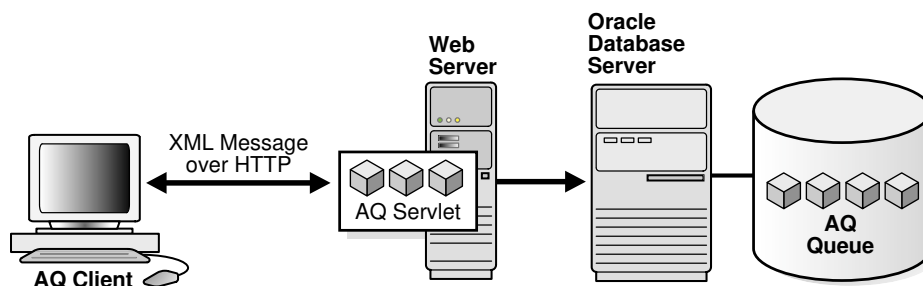
Figure 13-1 Architecture for Performing Oracle Database Advanced Queuing Operations Using HTTP
