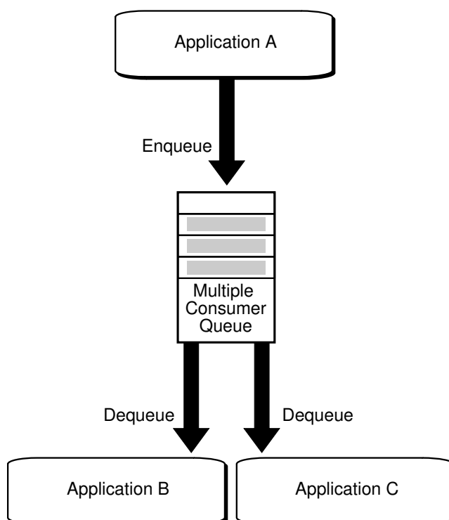
Figure 1-3 Communication Using a Multiconsumer Queue
