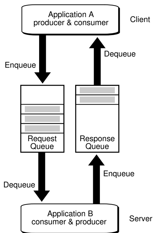
Figure 1-2 Client/Server Communication Using TEQ and AQ
