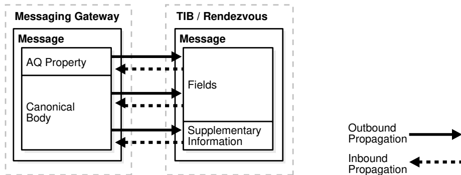
Figure C-5 Message Conversion for TIB/Rendezvous
