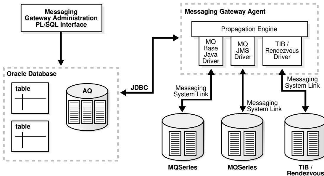
Figure C-1 Messaging Gateway Architecture
