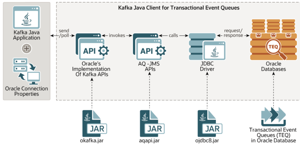
Figure 6-1 Kafka Application Integration with Transactional Event Queue
