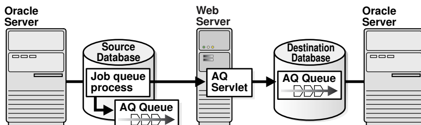
Figure 13-2 HTTP Oracle Database Advanced Queuing Propagation
