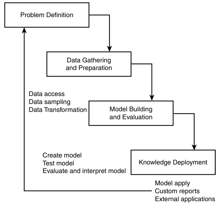
Figure 1-1 The Oracle Machine Learning Process
