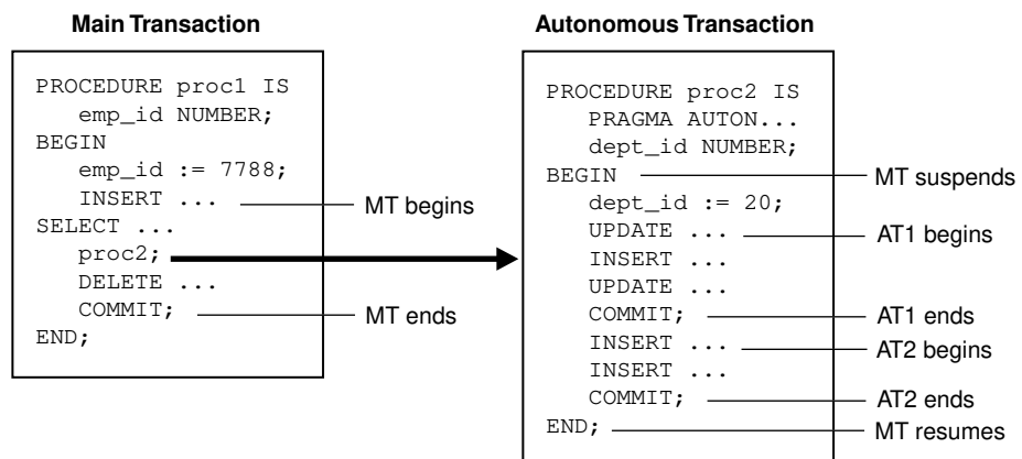
Figure 7-1 Transaction Control Flow
