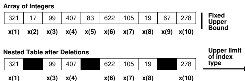
Figure 6-2 Array and Nested Table
