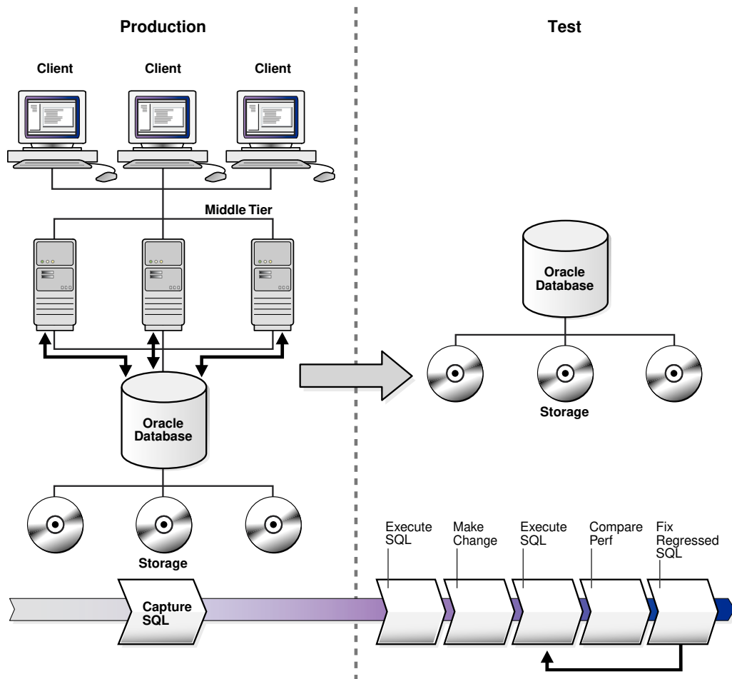
Figure 2-1 SQL Performance Analyzer Workflow
