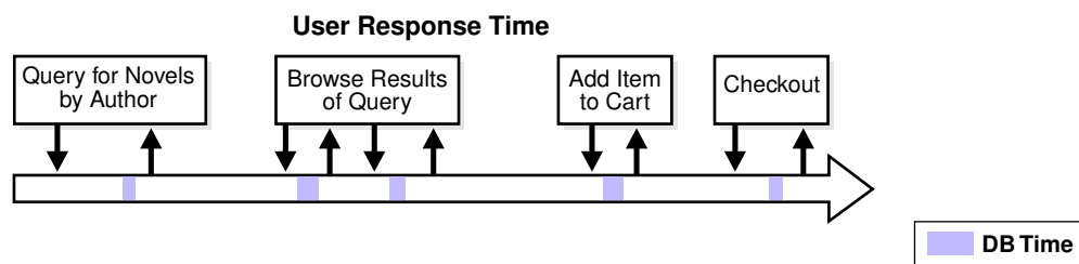
Figure 2-2 DB Time in User Transaction
