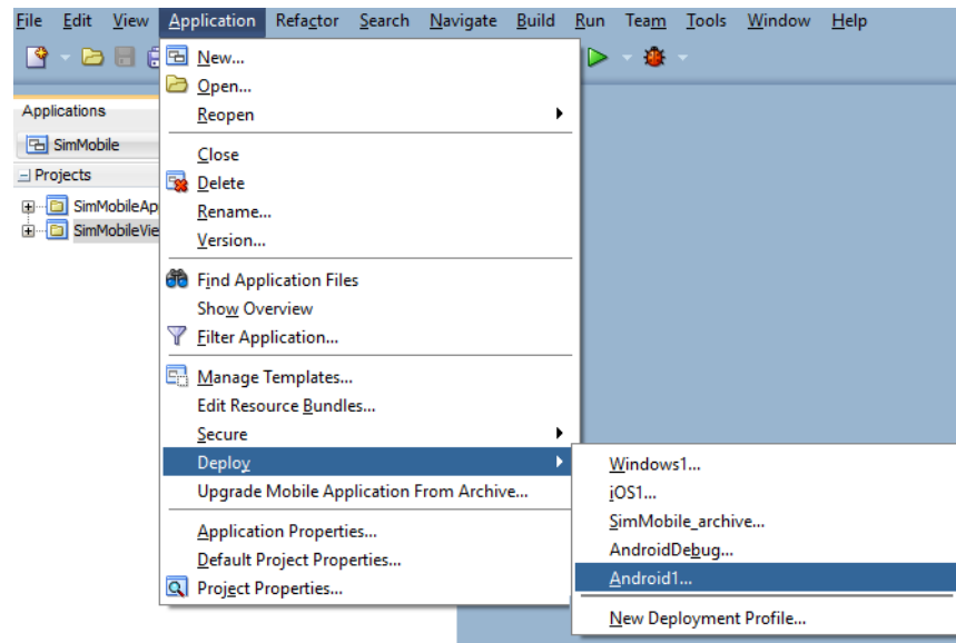
Figure 2–9 Deploy - Android1
