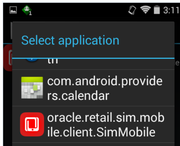
Figure 2–11 Associated Apps
