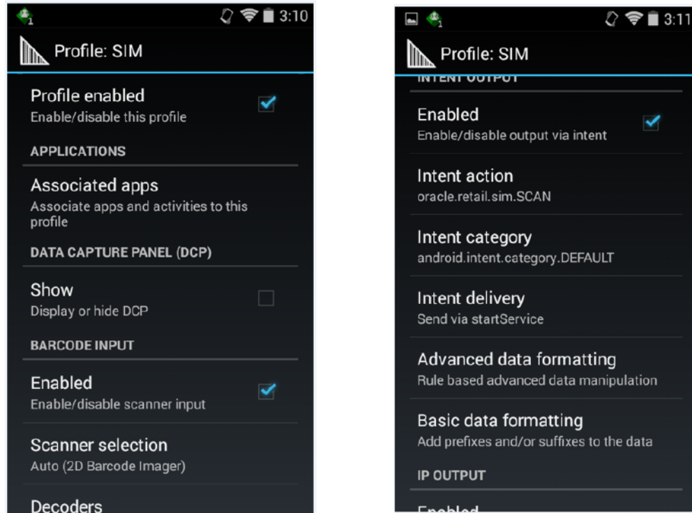
Figure 2–12 Profile Settings
