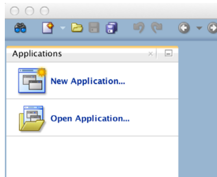
Figure 2-4 New Application
