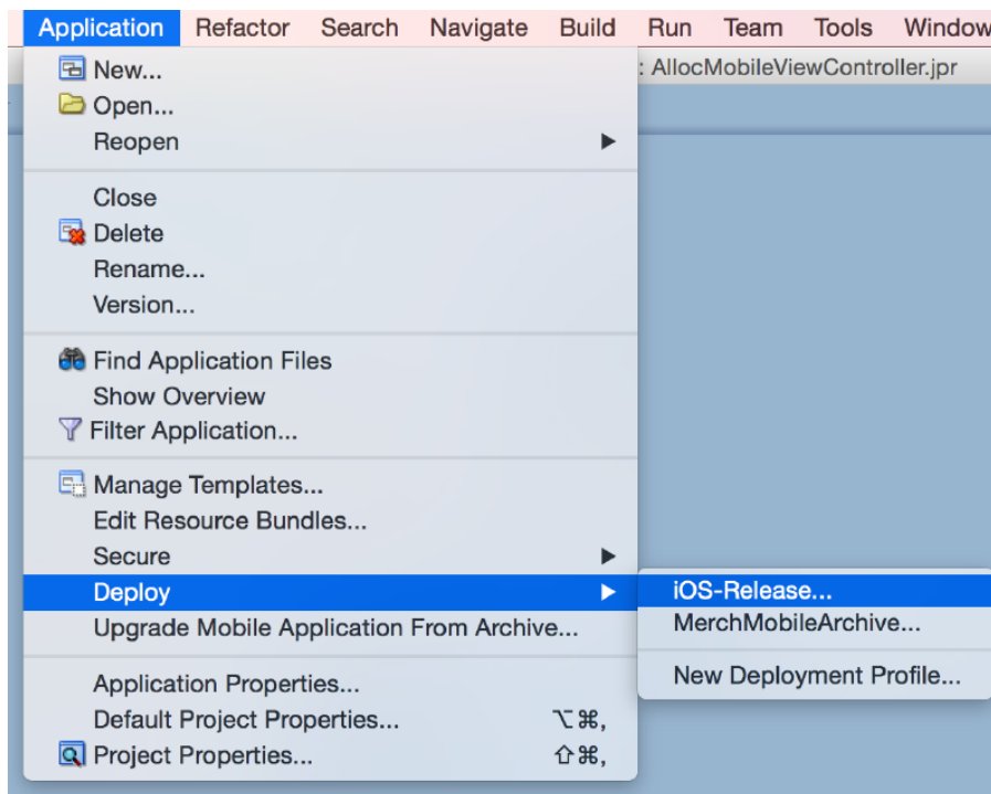
Figure 2-7 Deploy iOS-Release
