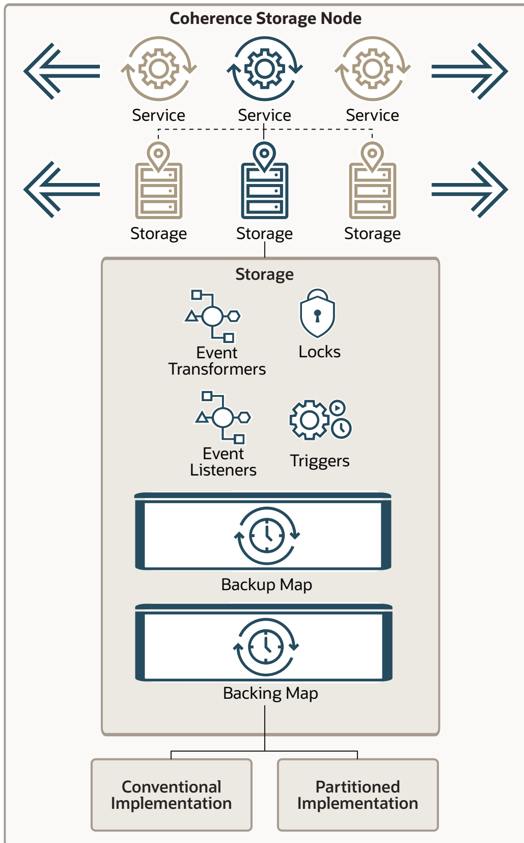
Figure 13-1 Backing Map Storage
