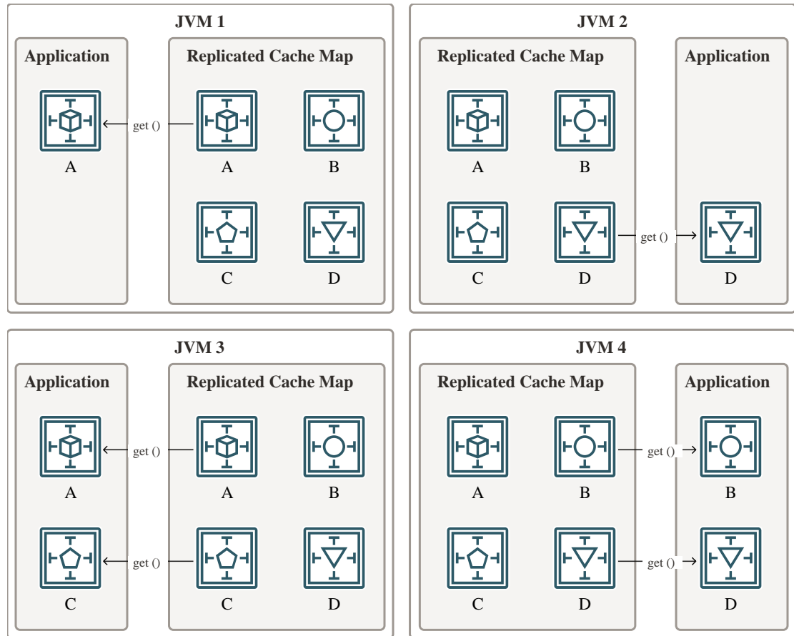
Figure 11-5 Get Operation in a Replicated Cache
