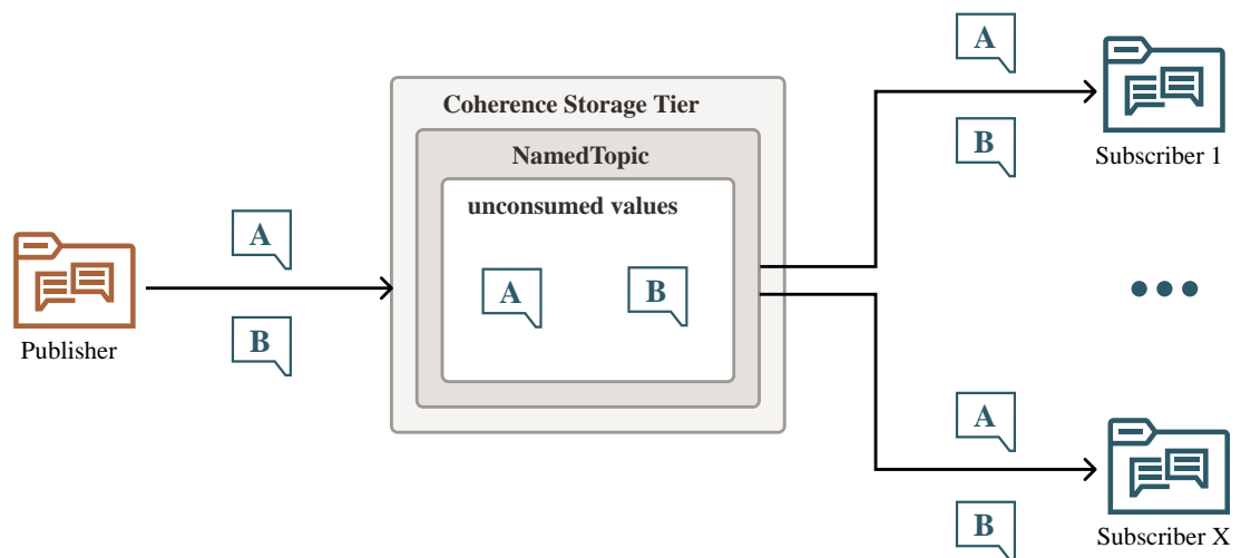
Figure 19-1 Topic Values
