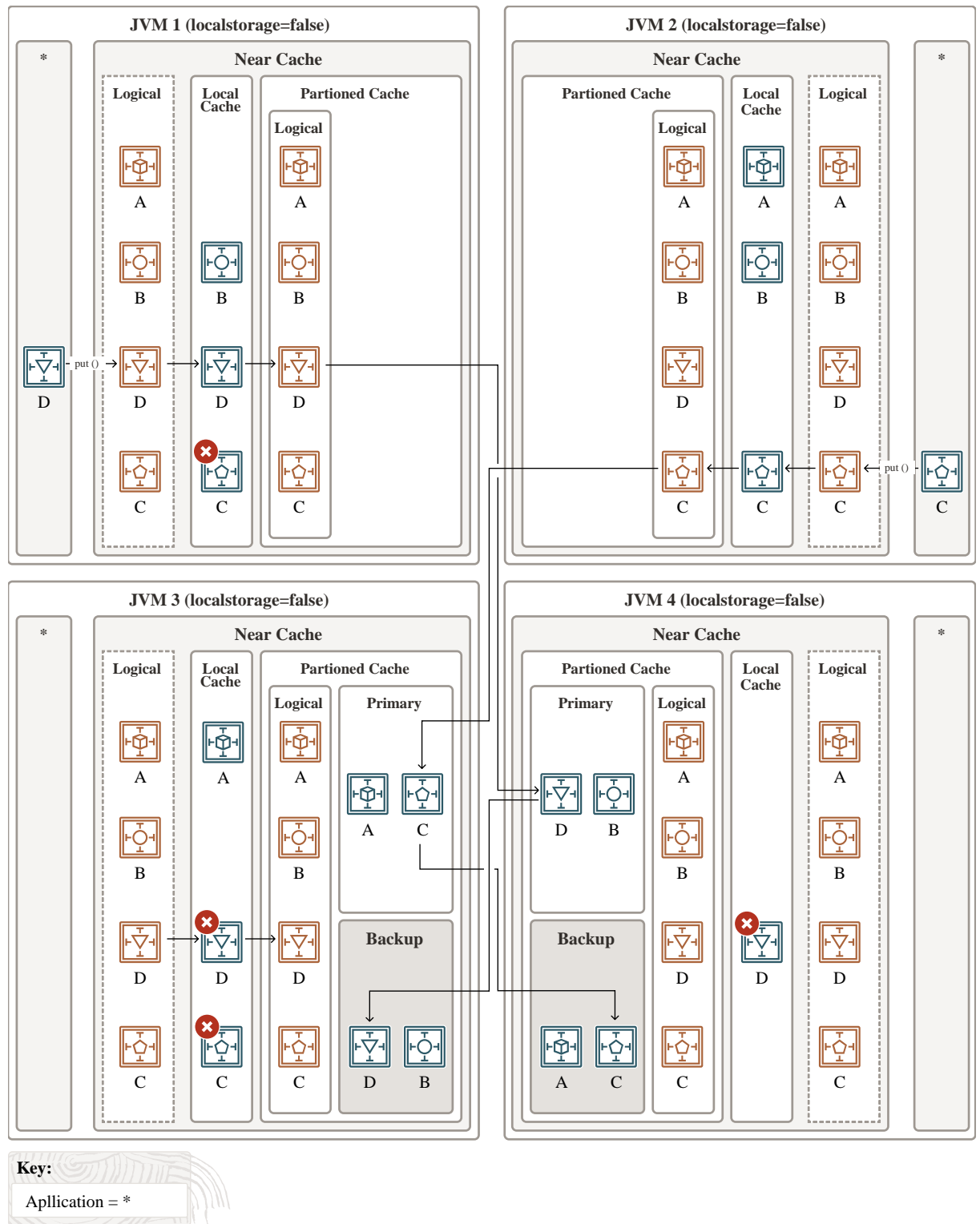
Figure 11-7 Put Operations in a Near Cache
