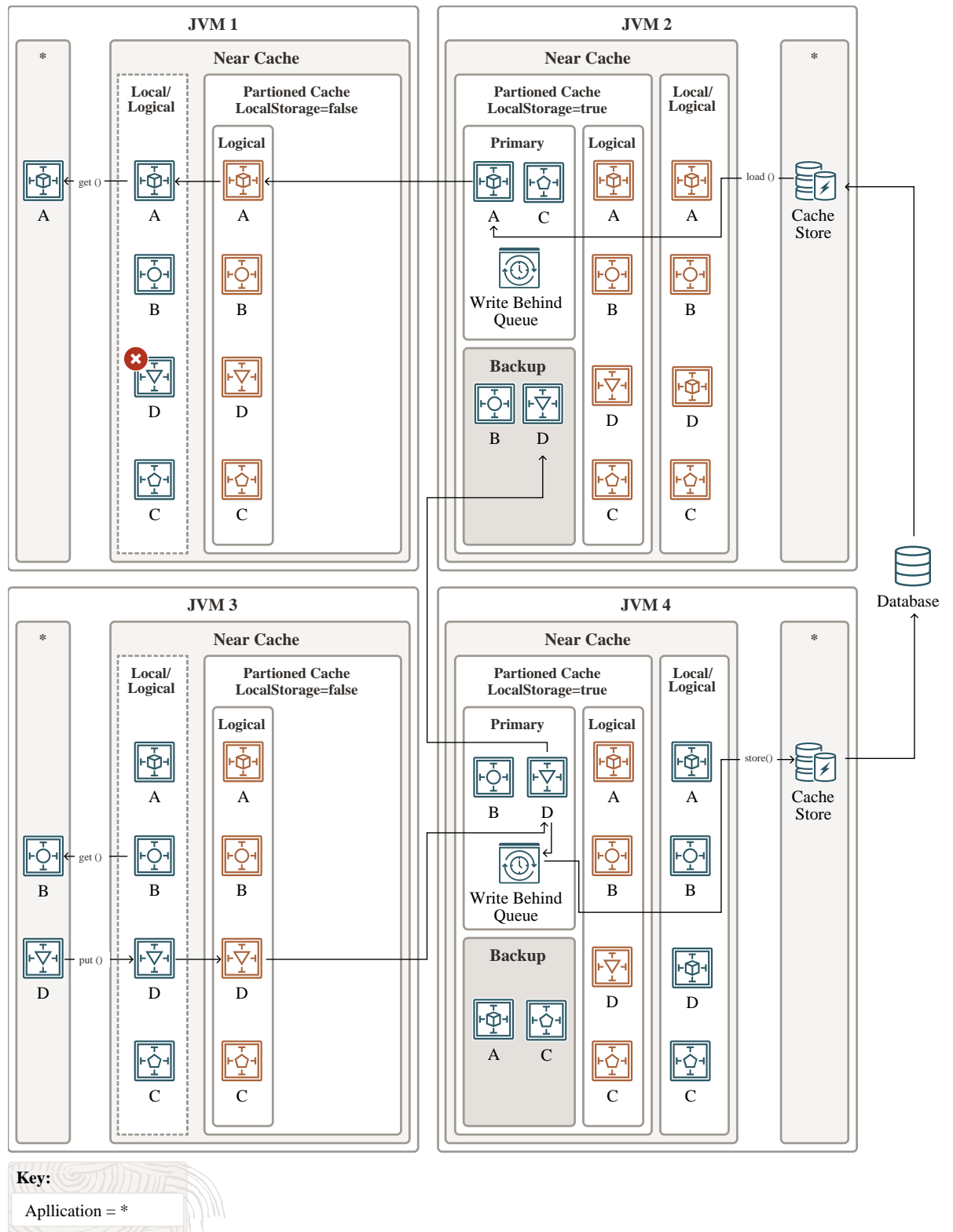
Figure 14-3 Write-Behind Caching
