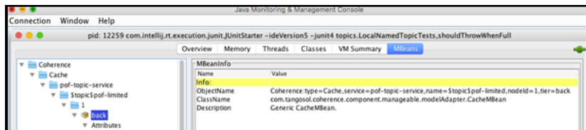
Figure 22-1 Topic pof-limited
