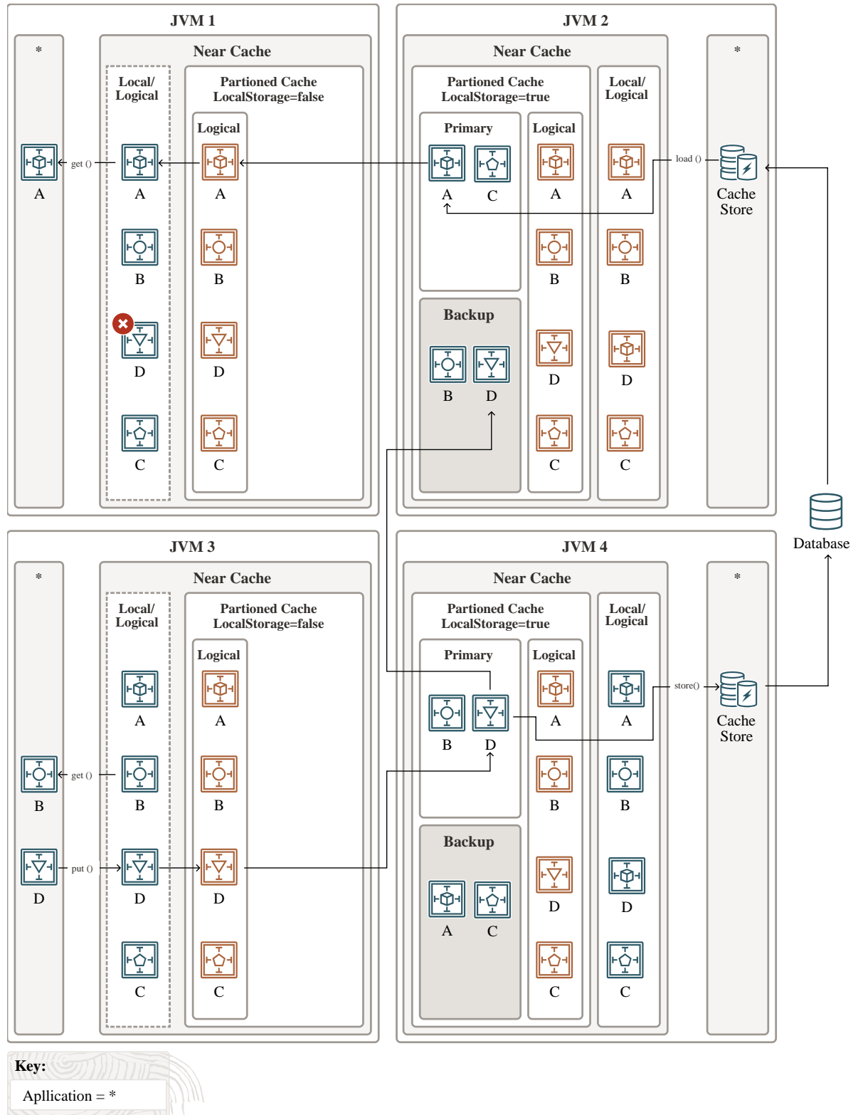
Figure 14-2 Write-Through Caching
