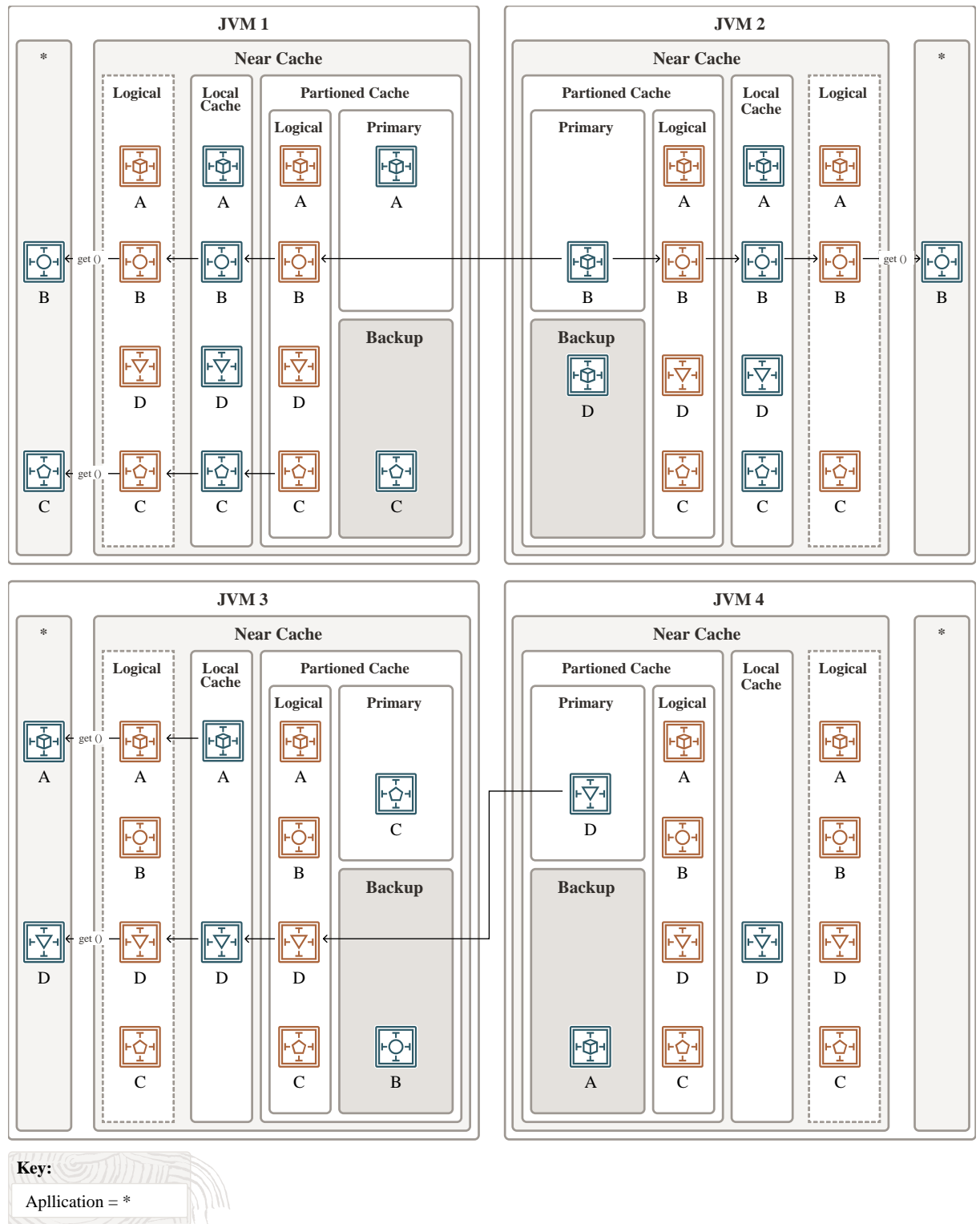
Figure 11-8 Get Operations in a Near Cache
