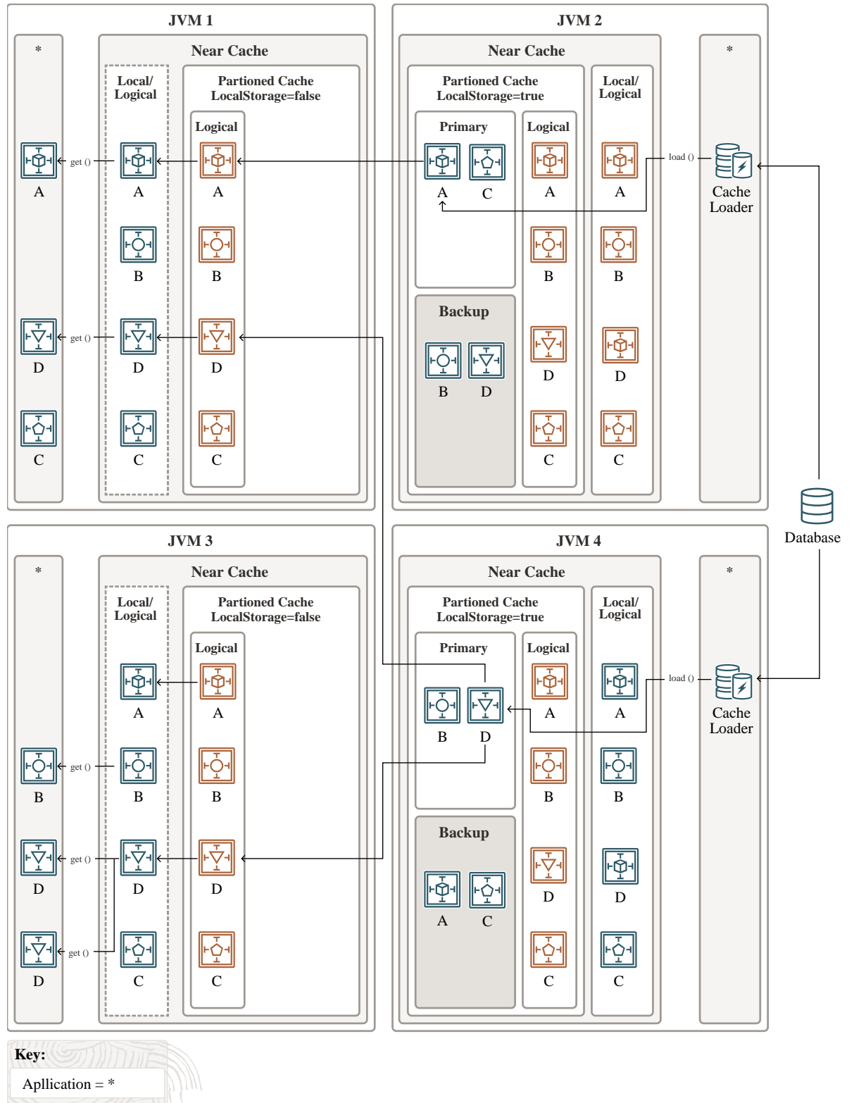
Figure 14-1 Read-Through Caching
