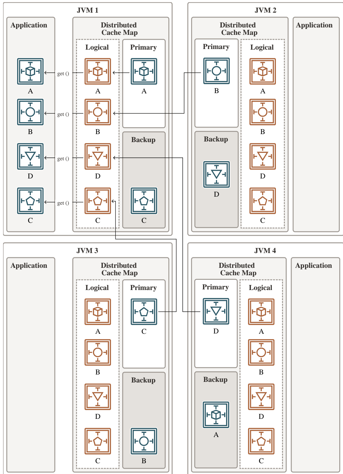
Figure 11-1 Get Operations in a Distributed Cache
