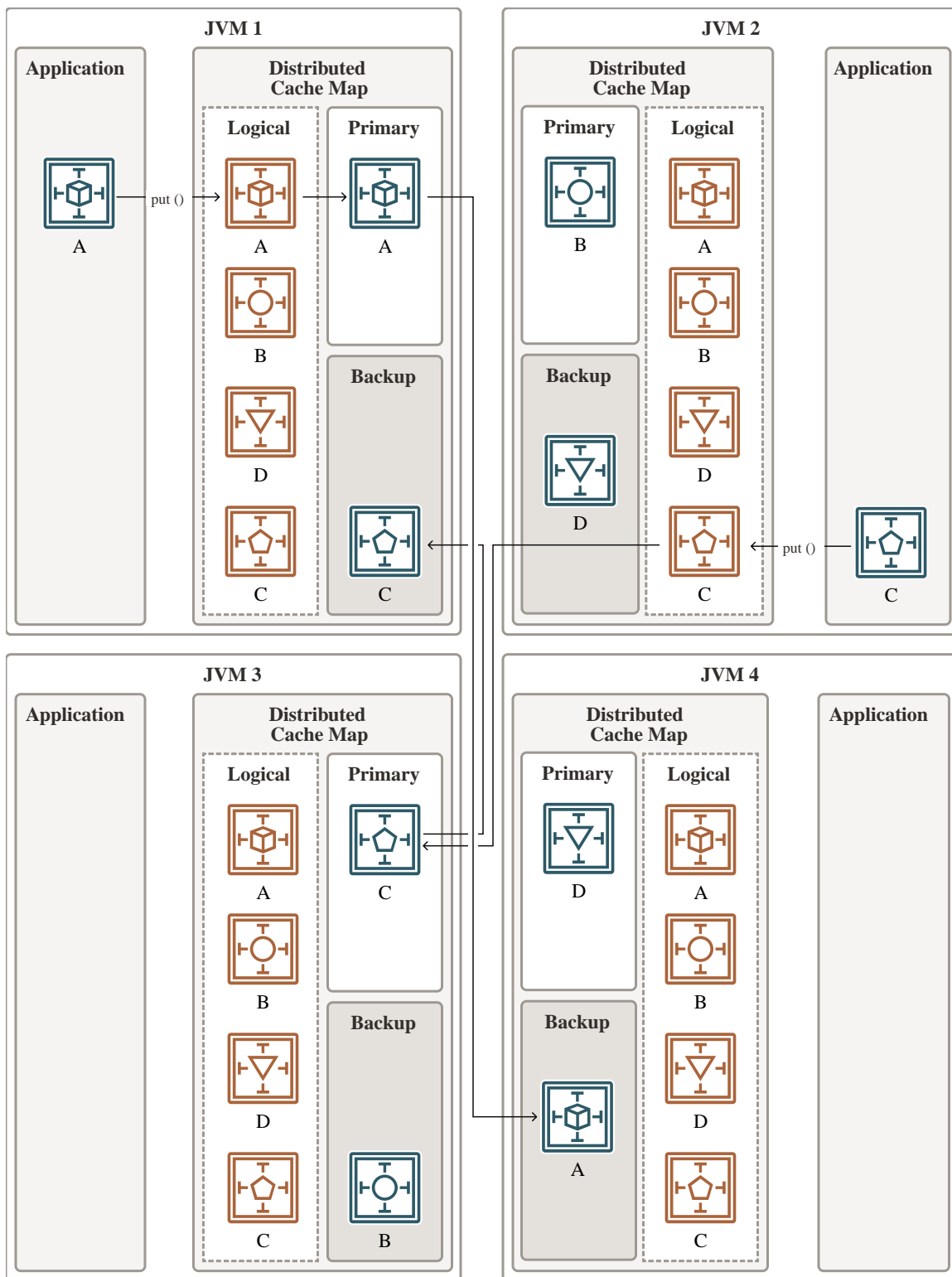
Figure 11-2 Put Operations in a distributed Cache Environment
