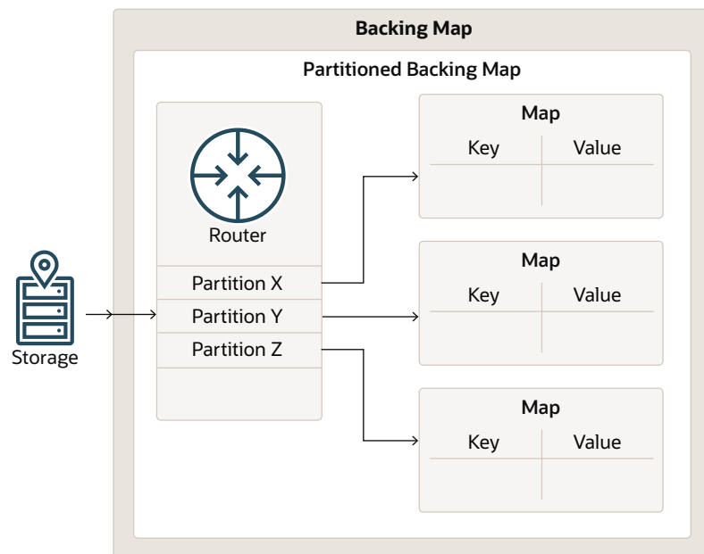
Figure 13-3 Partitioned Backing Map Implementation
