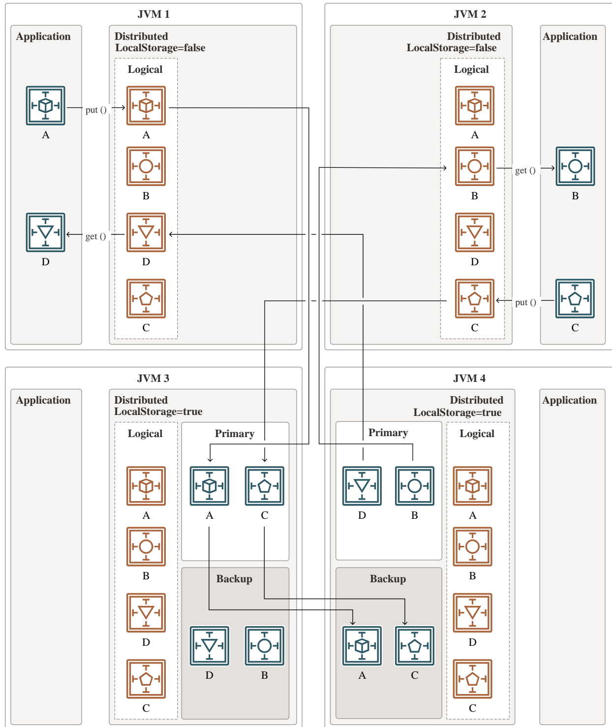
Figure 11-4 Local Storage in a Distributed Cache
