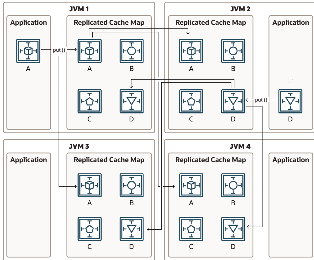
Figure 11-6 Put Operation in a Replicated Cache
