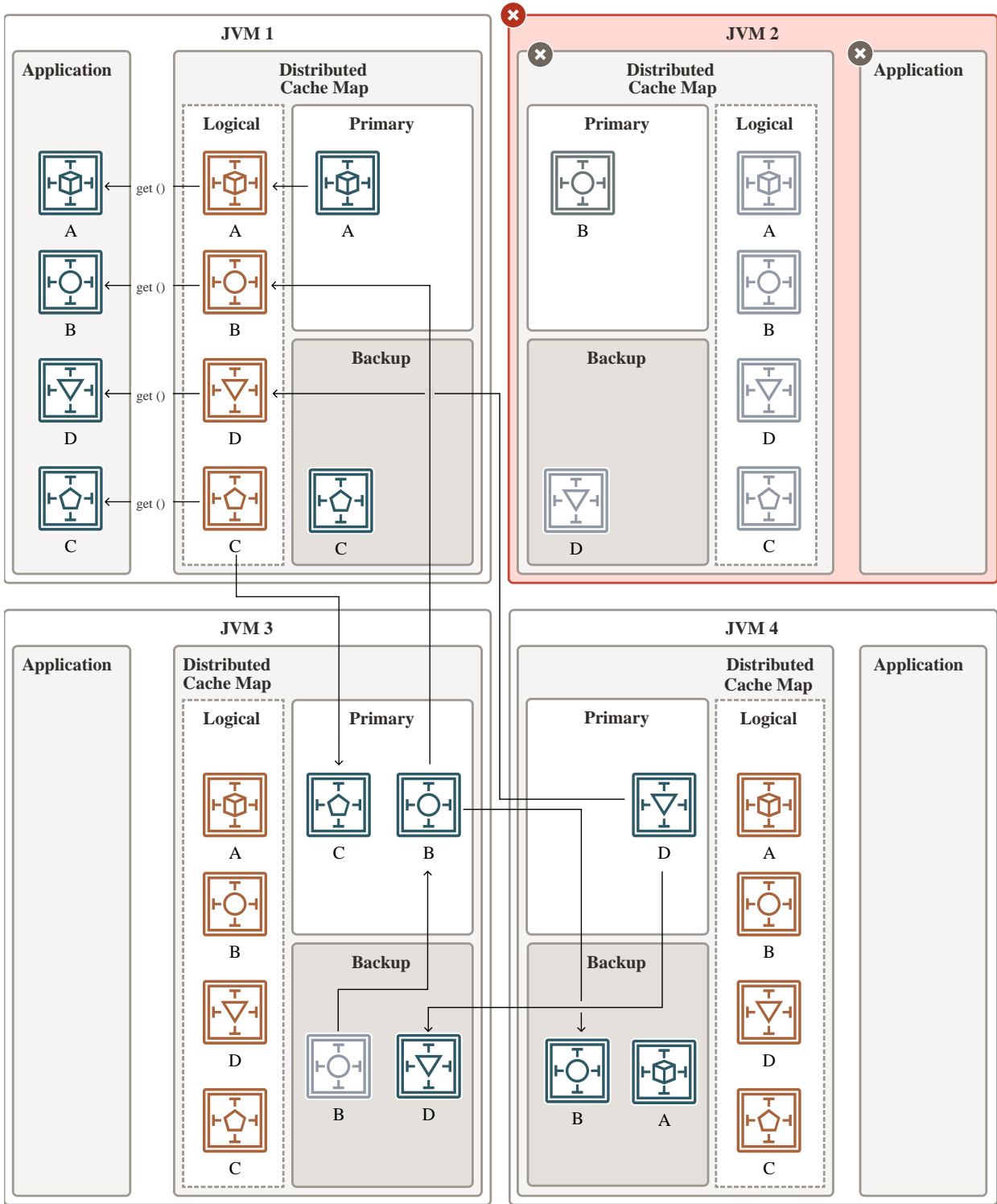
Figure 11-3 Failover in a Distributed Cache
