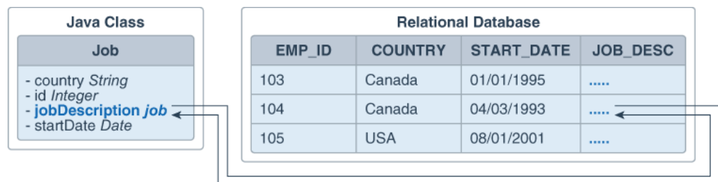
Figure 6-2 Serialized Object Converter (relational)
