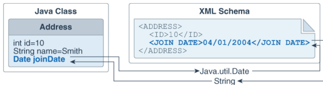
Figure 6-5 Type Conversion Mapping (nonrelational)
