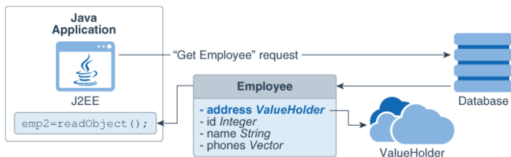
Figure 6-9 Address Object Not Read
