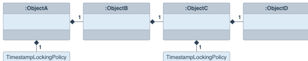
Figure 5-2 Optimistic Version Locking Policies and Cascading Example
