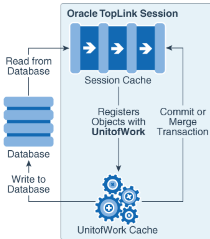
Figure 8-1 Object Life Cycle and the EclipseLink Caches
