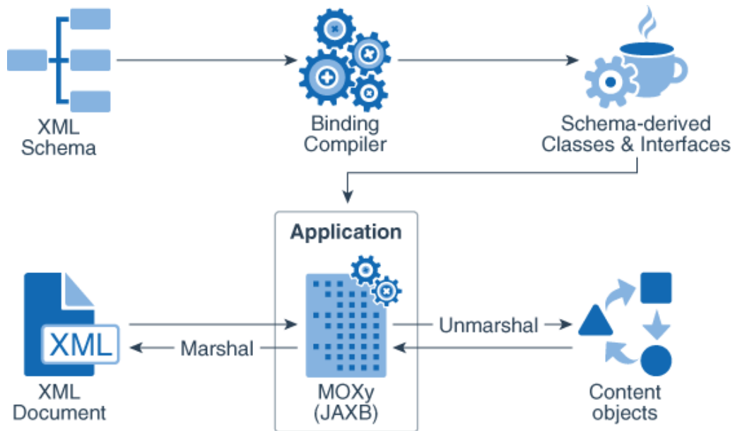
Figure 2-3 A Sample MOXy Architecture
