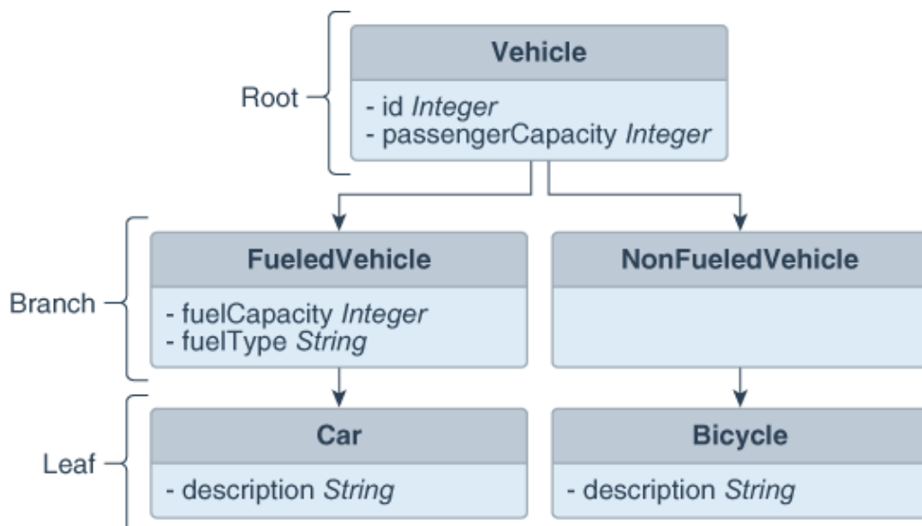
Figure 5-1 Example Inheritance Hierarchy
