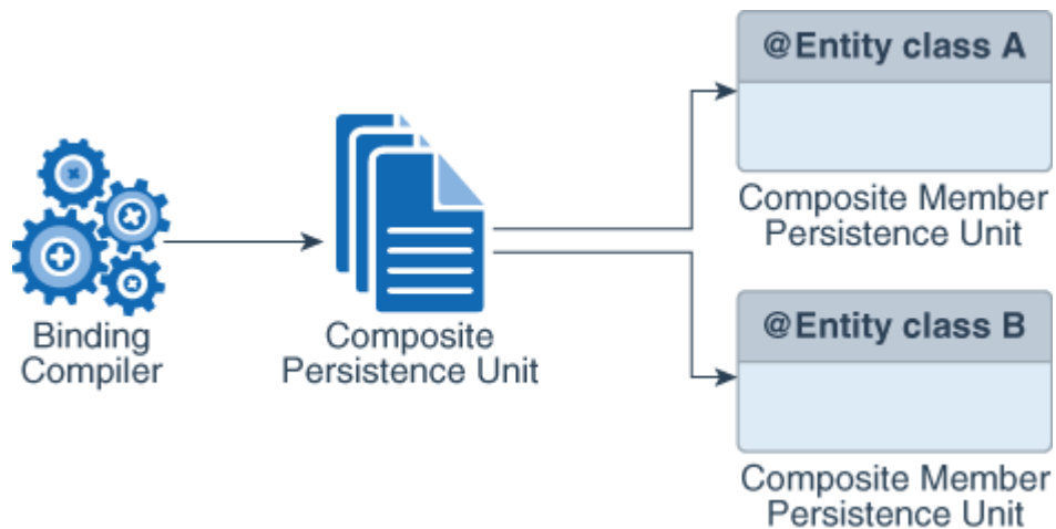
Figure 3-1 A Simple Composite Persistence Unit
