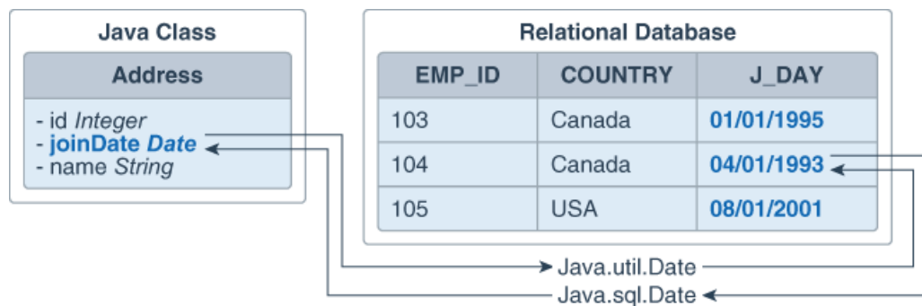
Figure 6-4 Type Conversion Mapping (relational)
