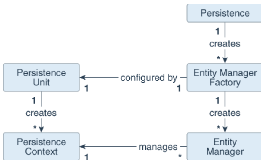
Figure 2-2 Relationships Between Entity Architecture Elements
