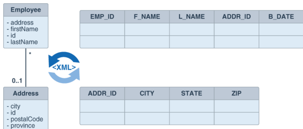
Figure 2-1 EclipseLink Metadata
