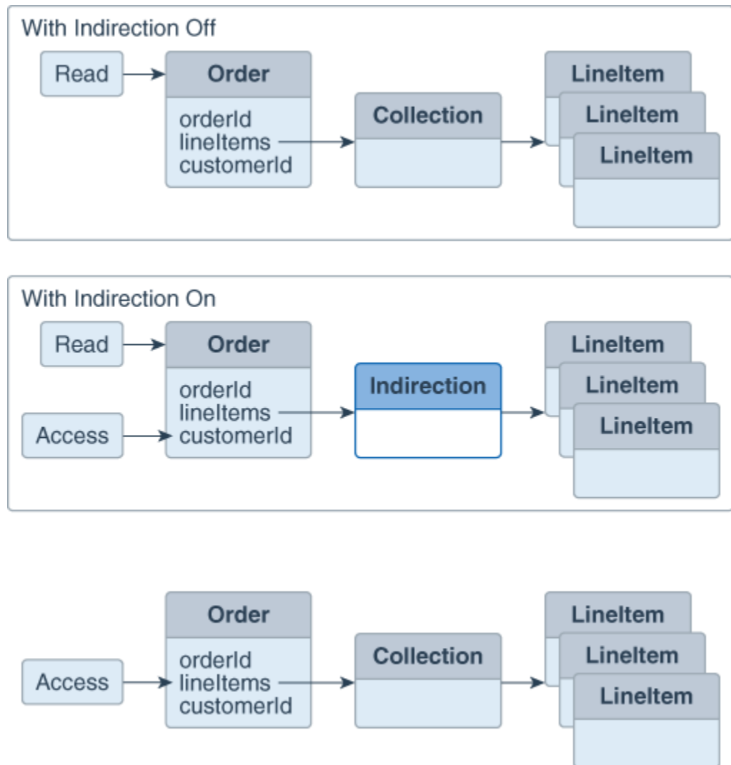
Figure 6-8 EclipseLink Indirection
