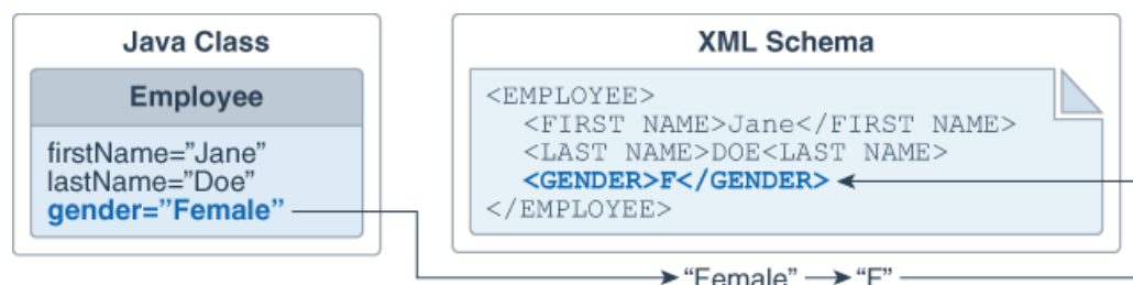
Figure 6-6 Object Type XML Converter
