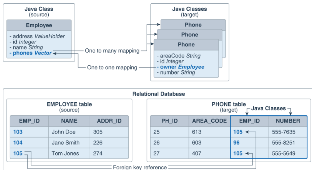
Figure 6-12 One-to-Many Relationships
