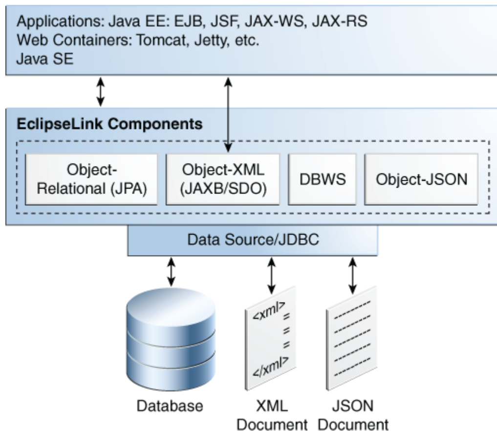
Figure 1-1 EclipseLink Components
