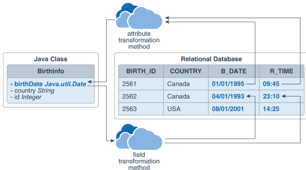
Figure 6-7 Transformation Mappings
