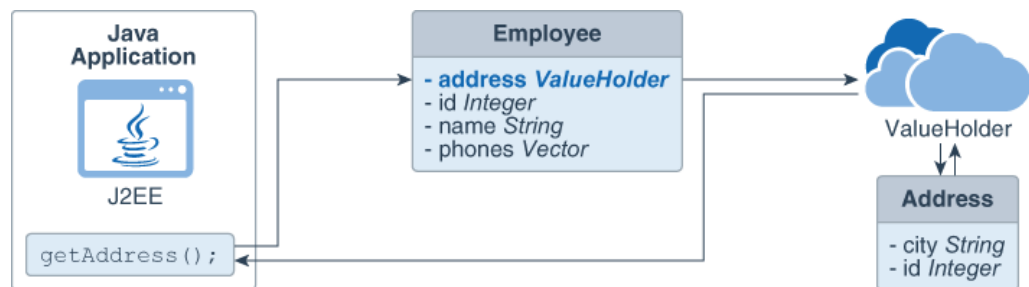
Figure 6-11 Subsequent Requests
