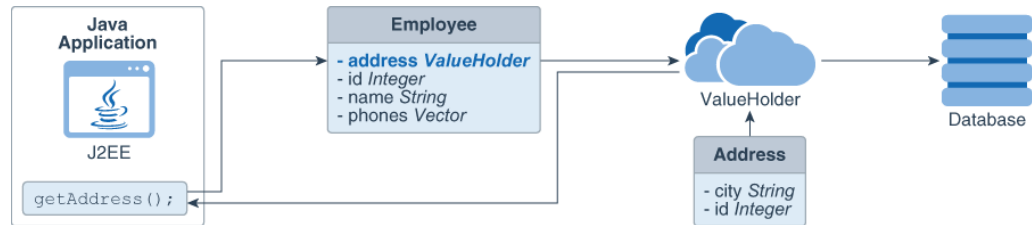
Figure 6-10 Initial Request
