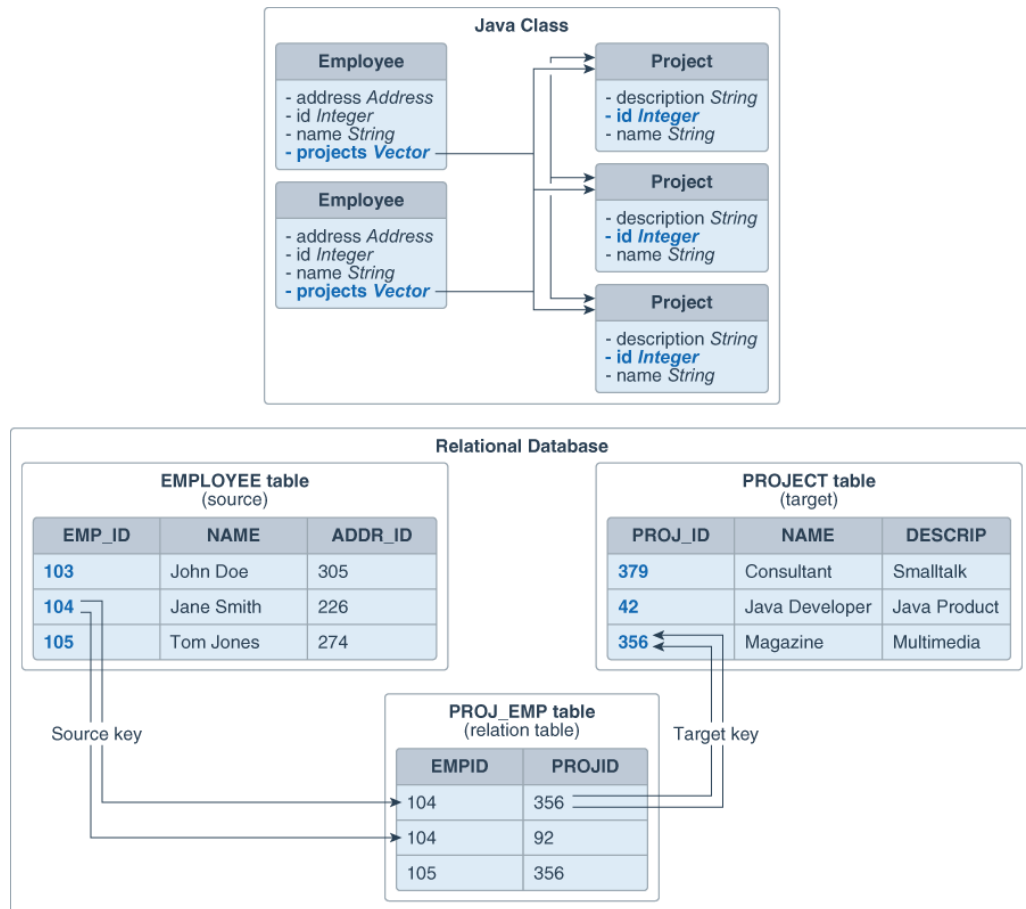
Figure 6-13 Many-to-Many Relationships
