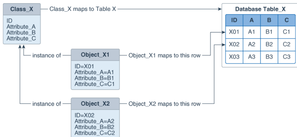
Figure 6-1 How Classes and Objects Map to a Database Table
