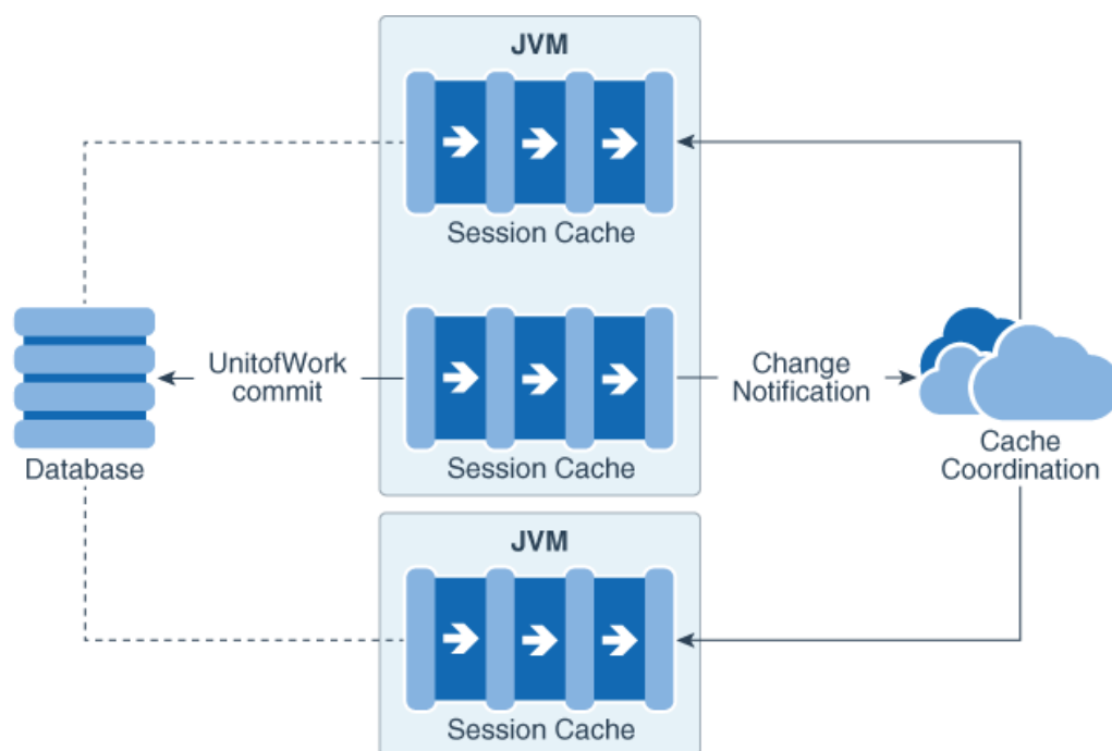
Figure 8-2 Coordinated Persistence Unit (Session) Caches
