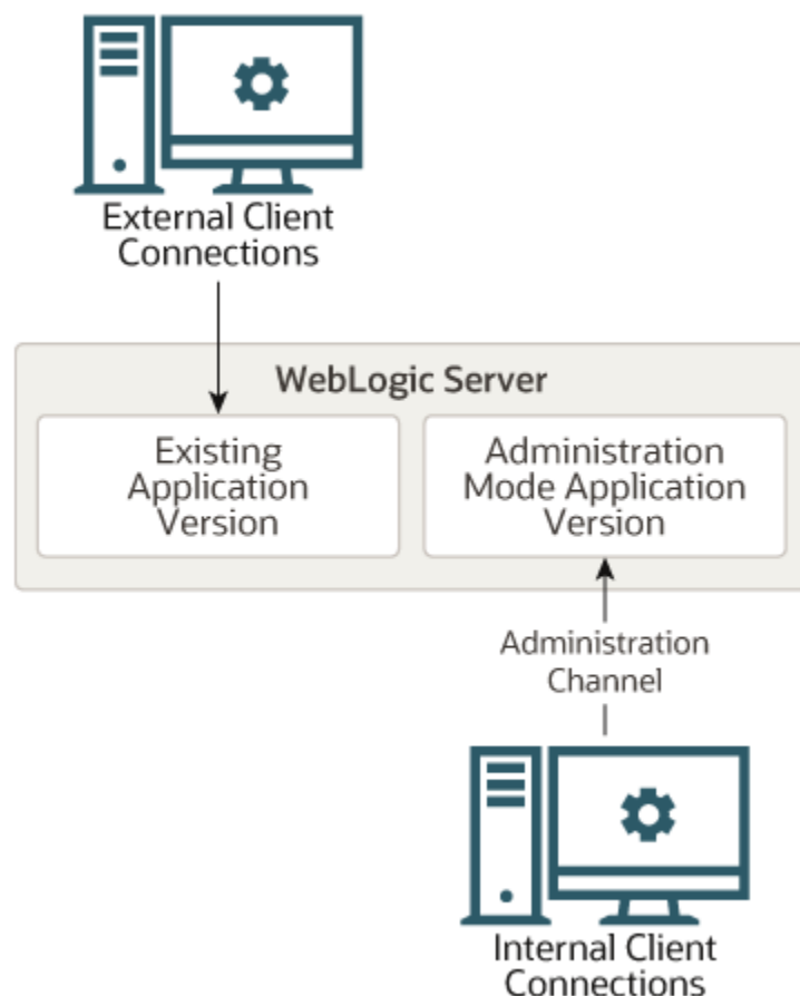
Figure 9-2 Distributing a New Version of an Application
