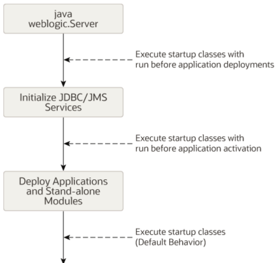
Figure 10-1 Startup Class Execution
