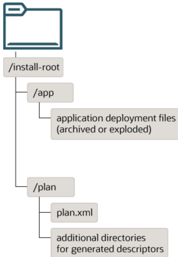
Figure 3-1 Application Installation Directory
