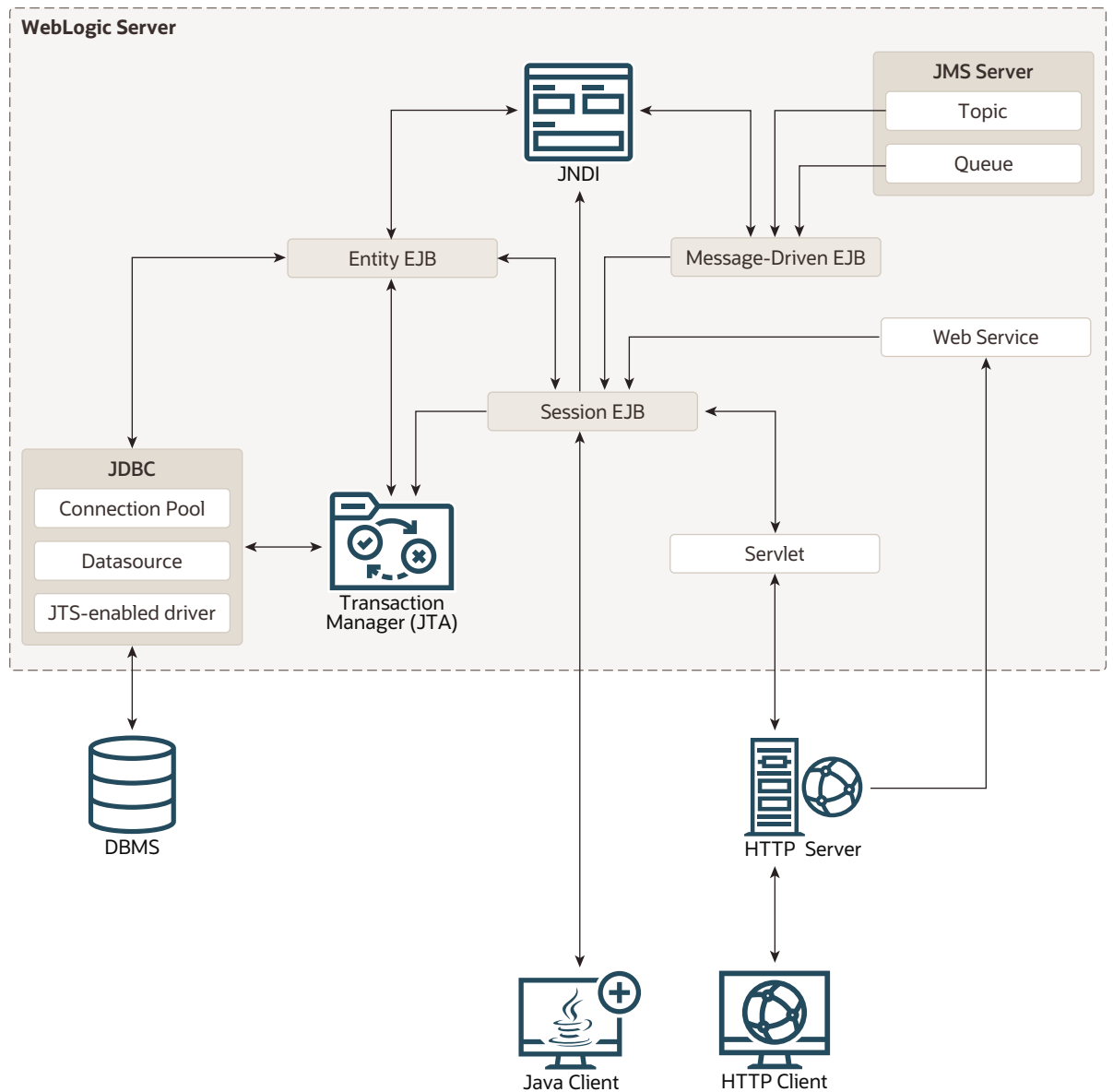
Figure 2-1 EJBs and Other Application Components
