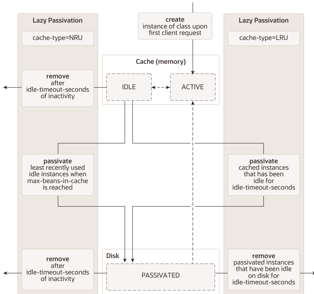
Figure 5-2 Stateful Session EJB Life Cycle
