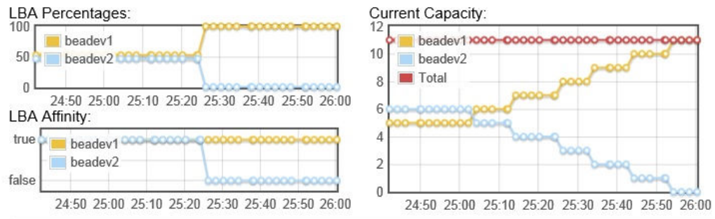
Figure 4-7 Gradual Draining
