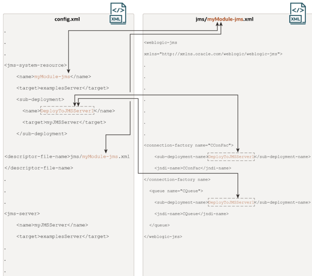
Figure 6-1 Subdeployment Architecture
