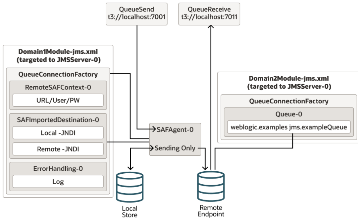
Figure 3-1 Store-and-Forward JMS Messages
