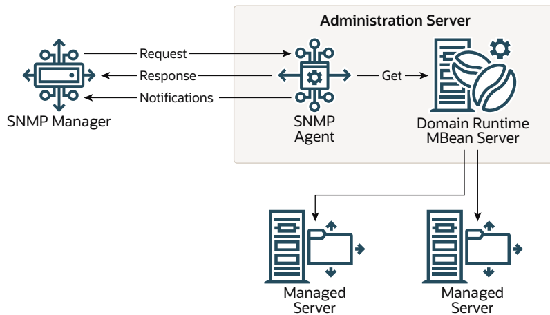
Figure 2-2 Centralized Model for SNMP Monitoring and Communication
