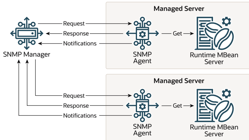
Figure 2-1 De-Centralized Model for SNMP Monitoring and Communication
