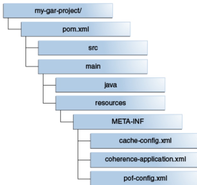
Figure 3-1 Maven Project Files
