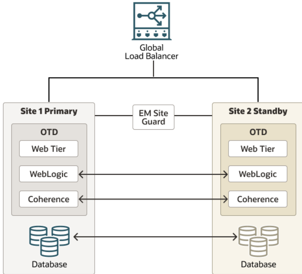
Figure 6-1 Domain Configuration for Active-Passive Recovery
