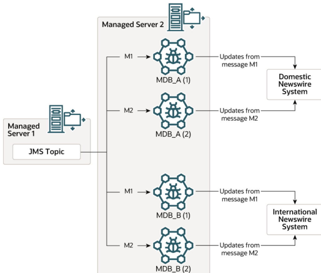
Figure 3-2 Publish/Subscribe Model
