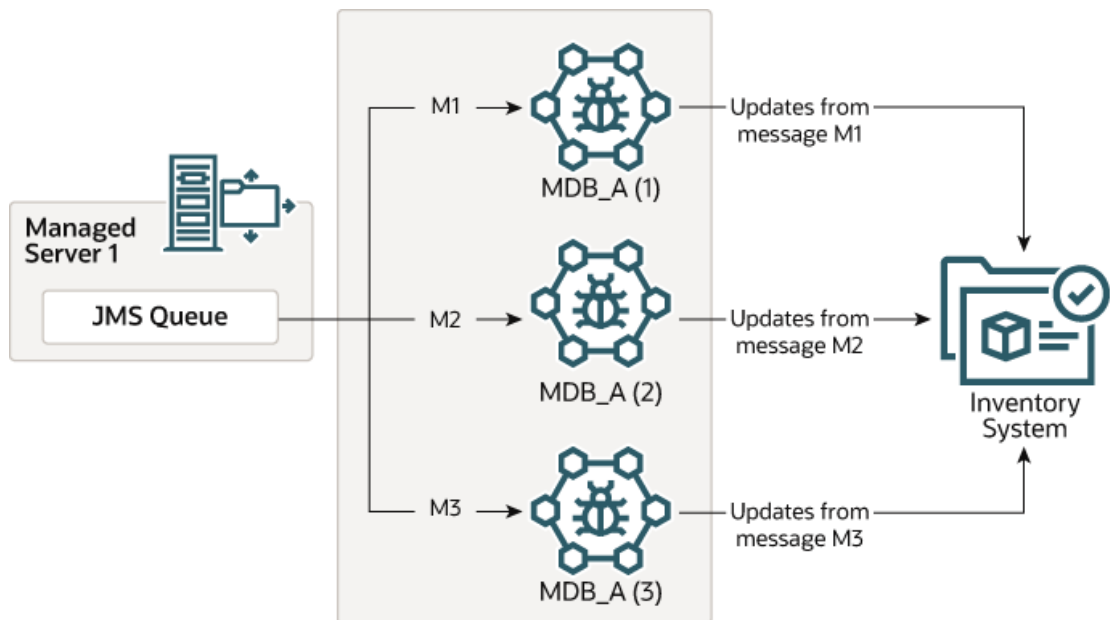
Figure 3-1 Point-to-Point Model
