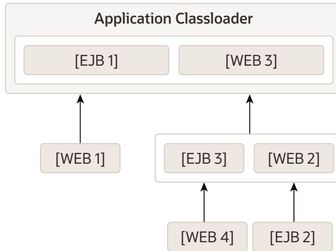
Figure 12-3 Example Classloader Hierarchy
