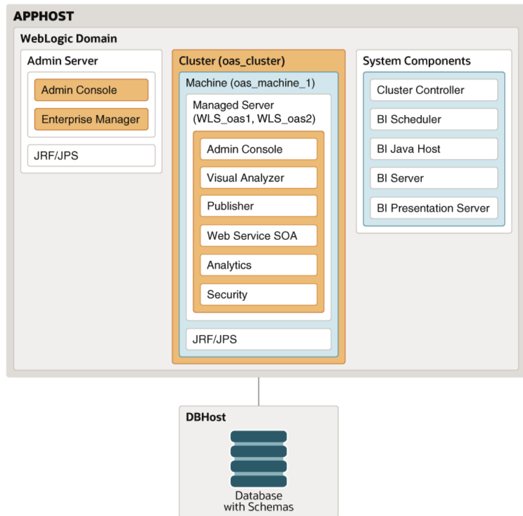
Figure 1-1 Oracle Analytics Server Standard Upgrade Topology
