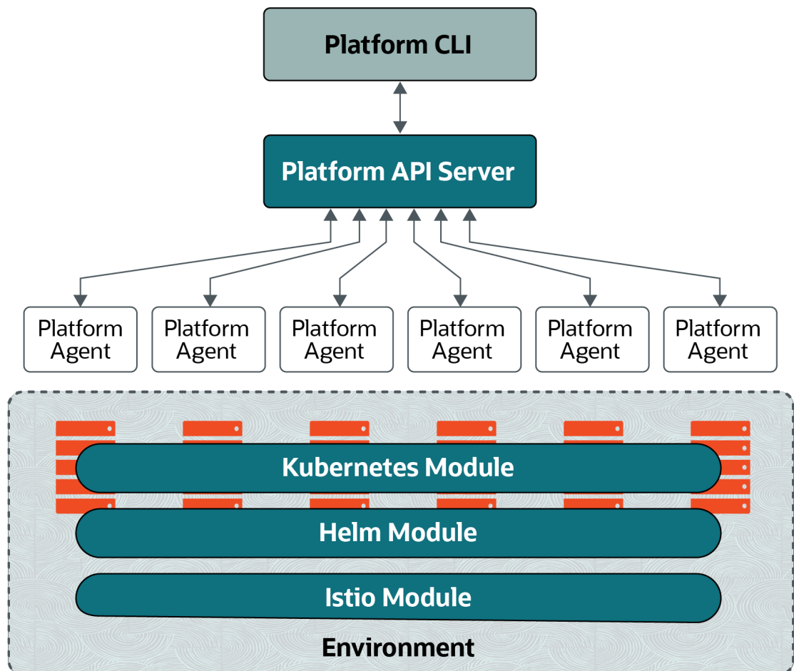
Figure 4-4 Istio module
