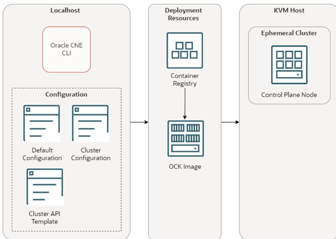
Figure 5-2 libvirt Ephemeral Cluster
