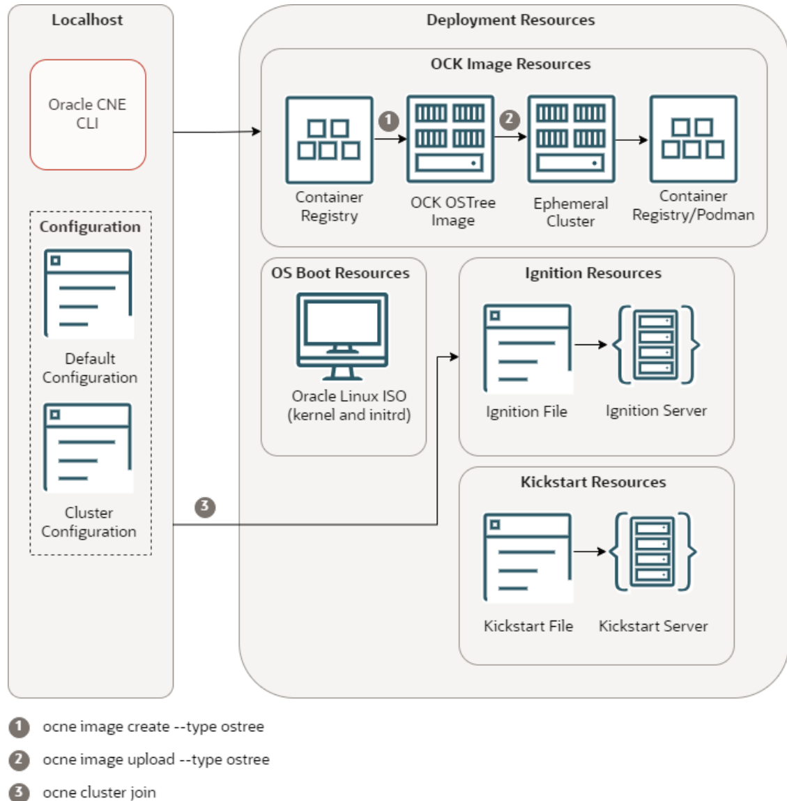
Figure 7-2 OCK Images in a Bring Your Own Cluster
