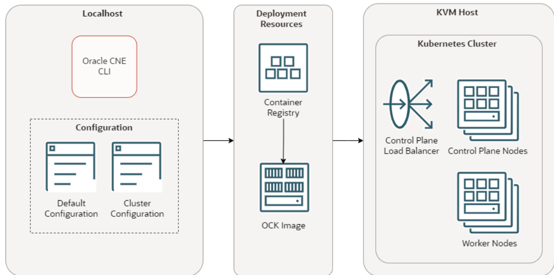
Figure 5-1 libvirt Cluster Architecture
