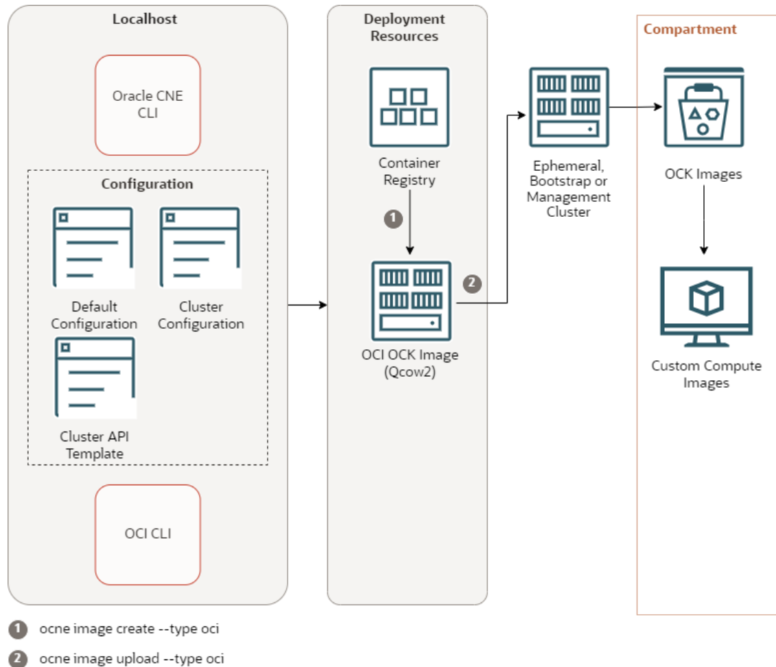
Figure 6-2 OCK Images for an OCI Cluster
