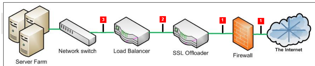
Figure R-1 Placement of Monitoring Device
