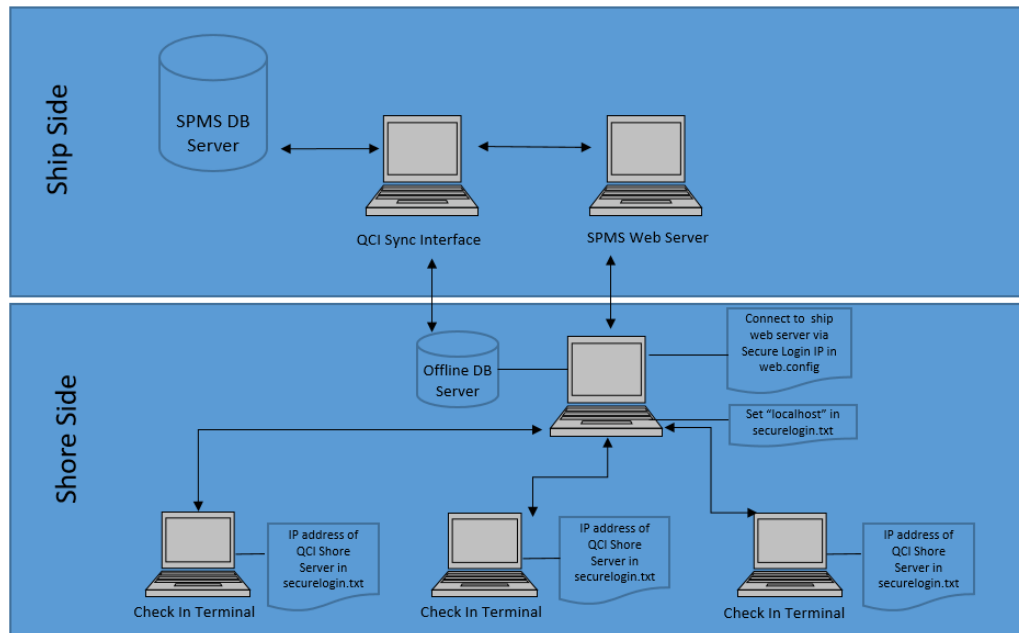
Figure 2-1 Environment Setup
