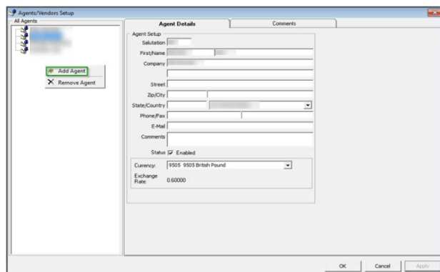
Figure 3-1 Vendor/Agent Setup
