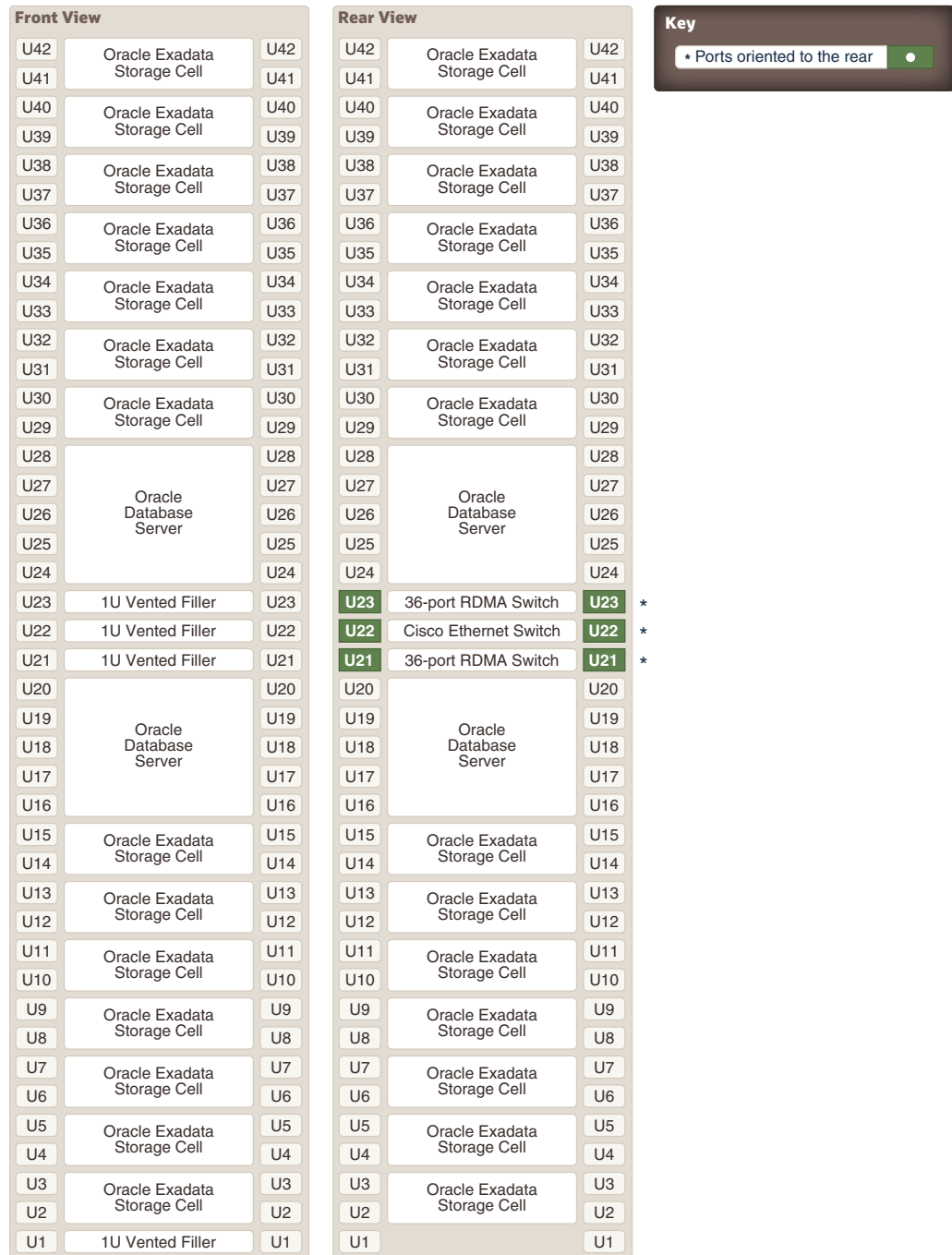
Figure 9-2 Rack Layout of Oracle Exadata Database Machine X8M-8
