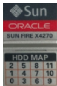
Figure 6-2 Disk Layout in Exadata Storage Server with Sun Fire X4270 M2 Servers
