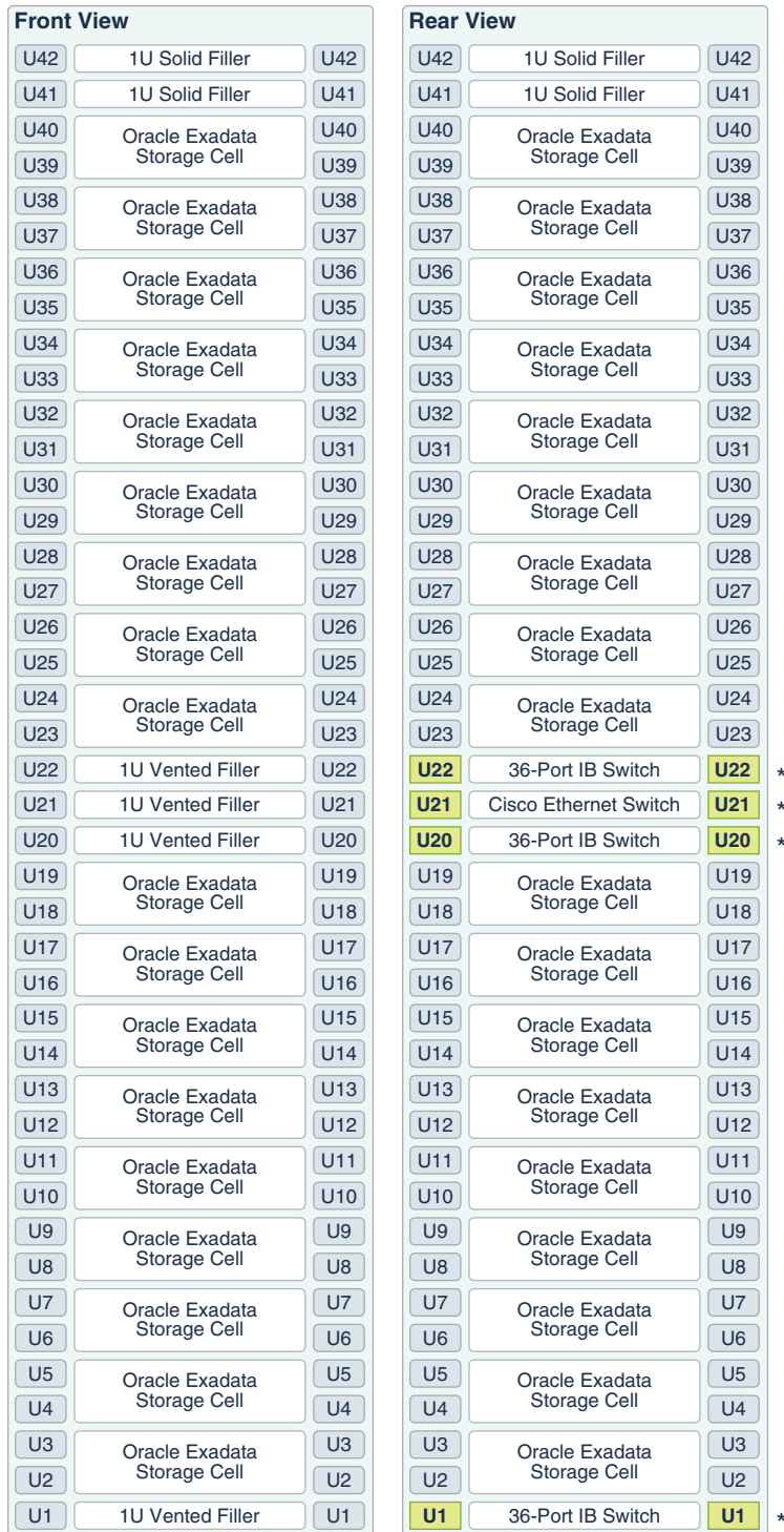
Figure 15-1 Rack Layout of Oracle Exadata Storage Expansion Full Rack X5 and Later
