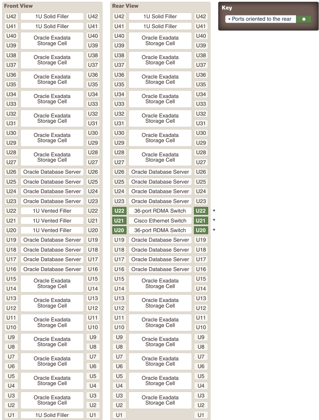
Figure 9-1 Rack Layout of Oracle Exadata Database Machine X8M-2 Full Rack
