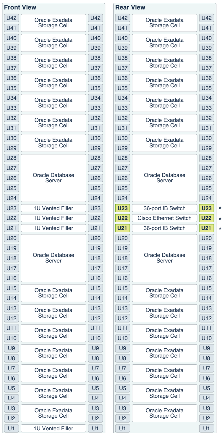
Figure 10-2 Rack Layout of Oracle Exadata Database Machine X8-8 and X7-8
