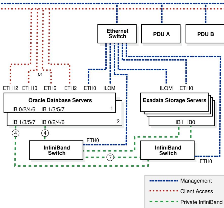
Figure 2-4 Network for Oracle Exadata Database Machine X8-8, X7-8, X6-8, X5-8, and X4-8 Full Rack with Bonded Client Access
