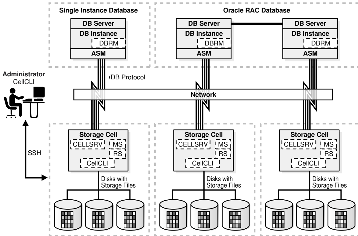
Figure 1-4 Software Components in the Oracle Exadata Database Machine Environment
