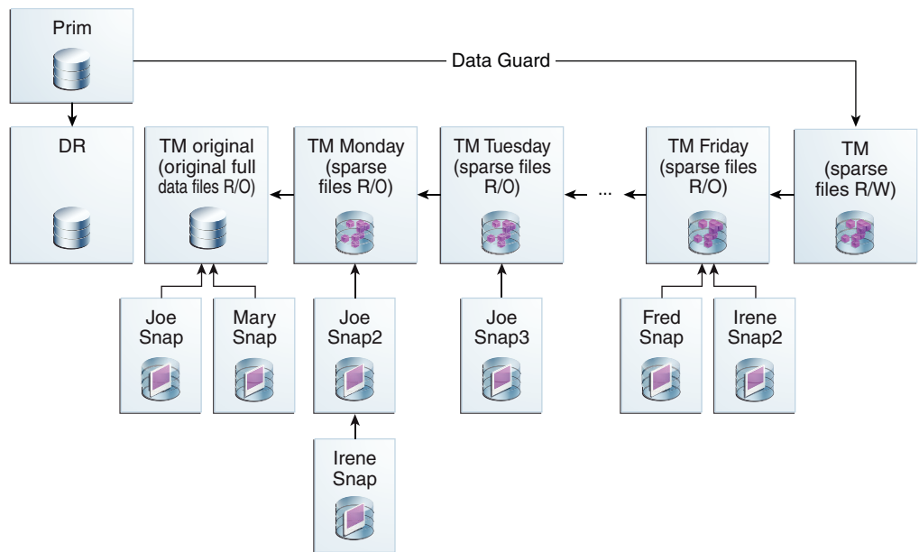
Figure 10-18 Potential Future Configuration
