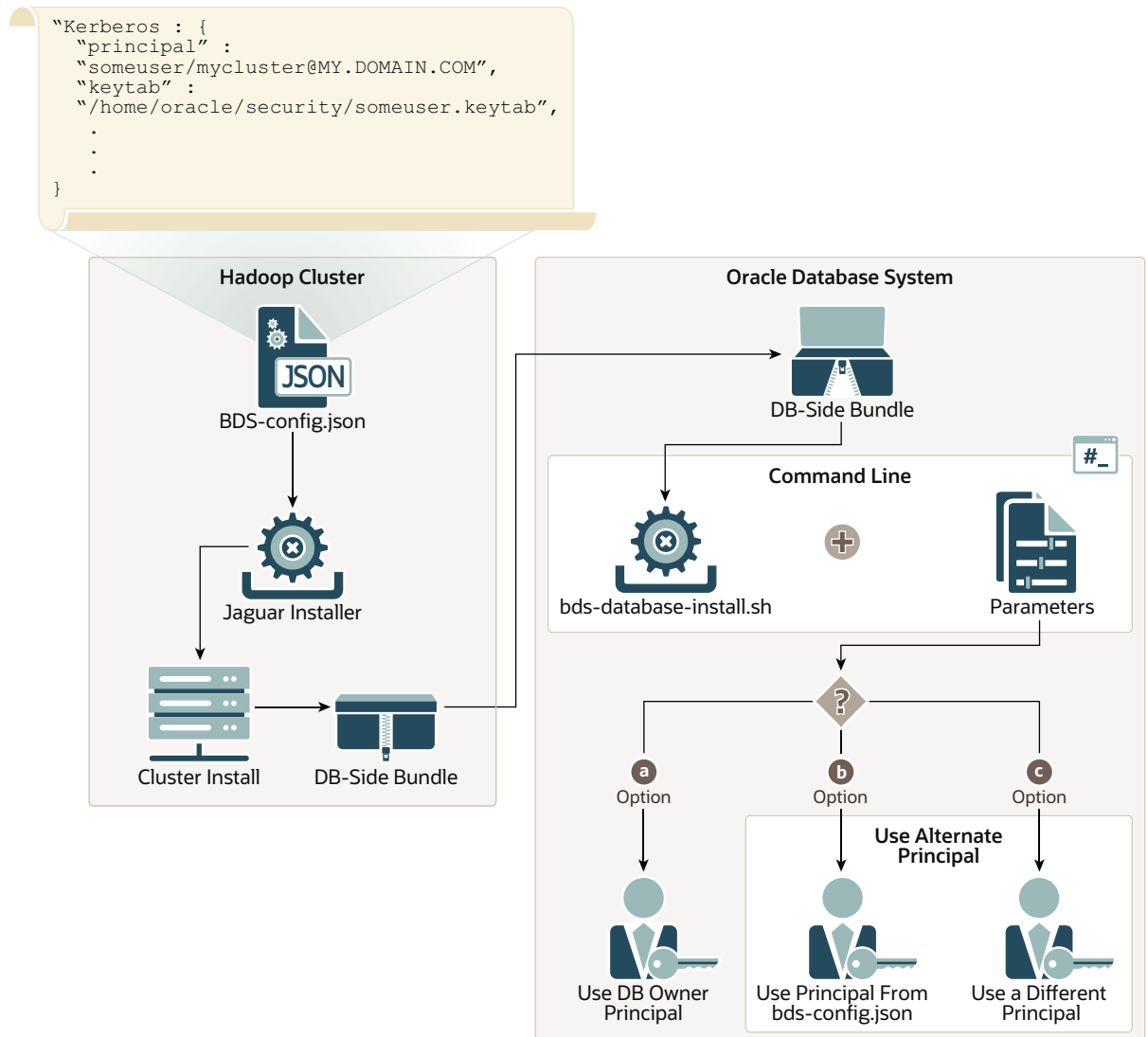
Figure 3-1 Using the --alternate-principal Parameter with bds-database-install.sh
