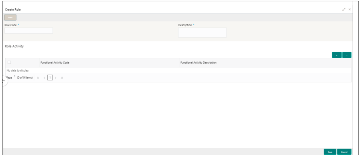
Figure 31: Create Role
