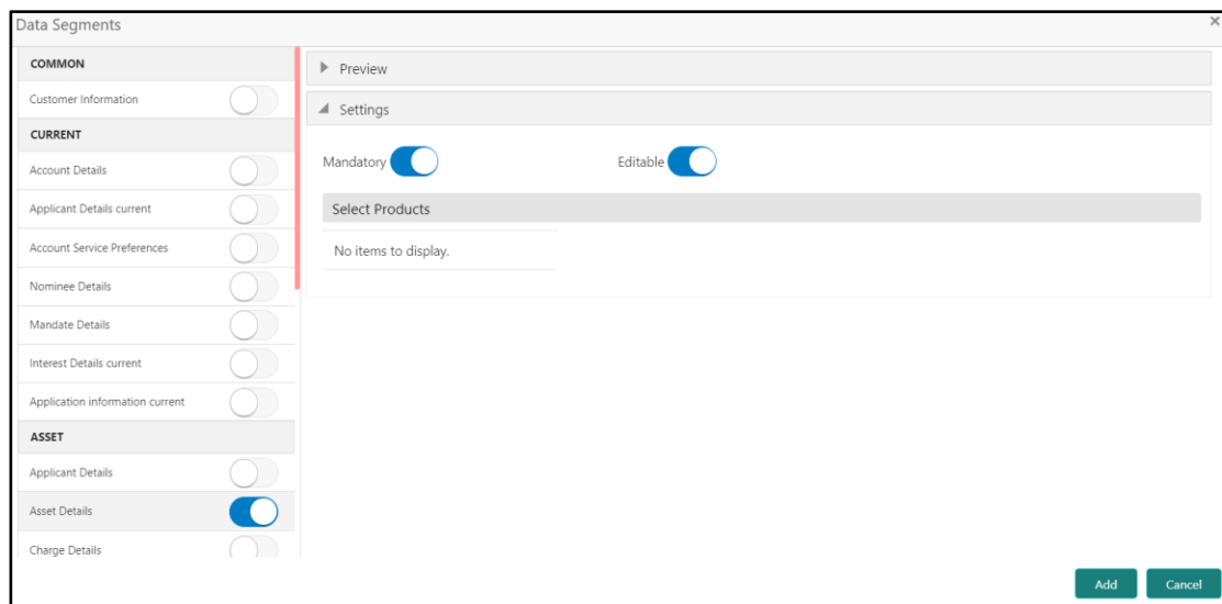
Figure 13: Data Segments
